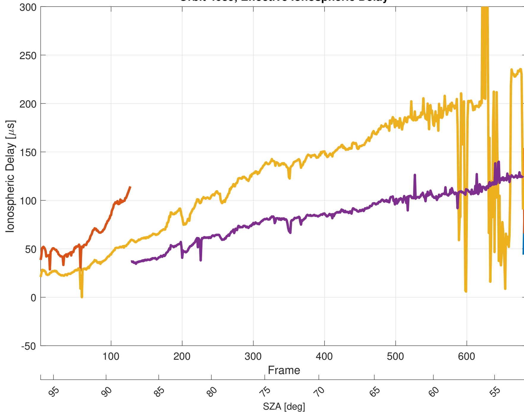
Orbit 4689, Effective Ionospheric Delay
