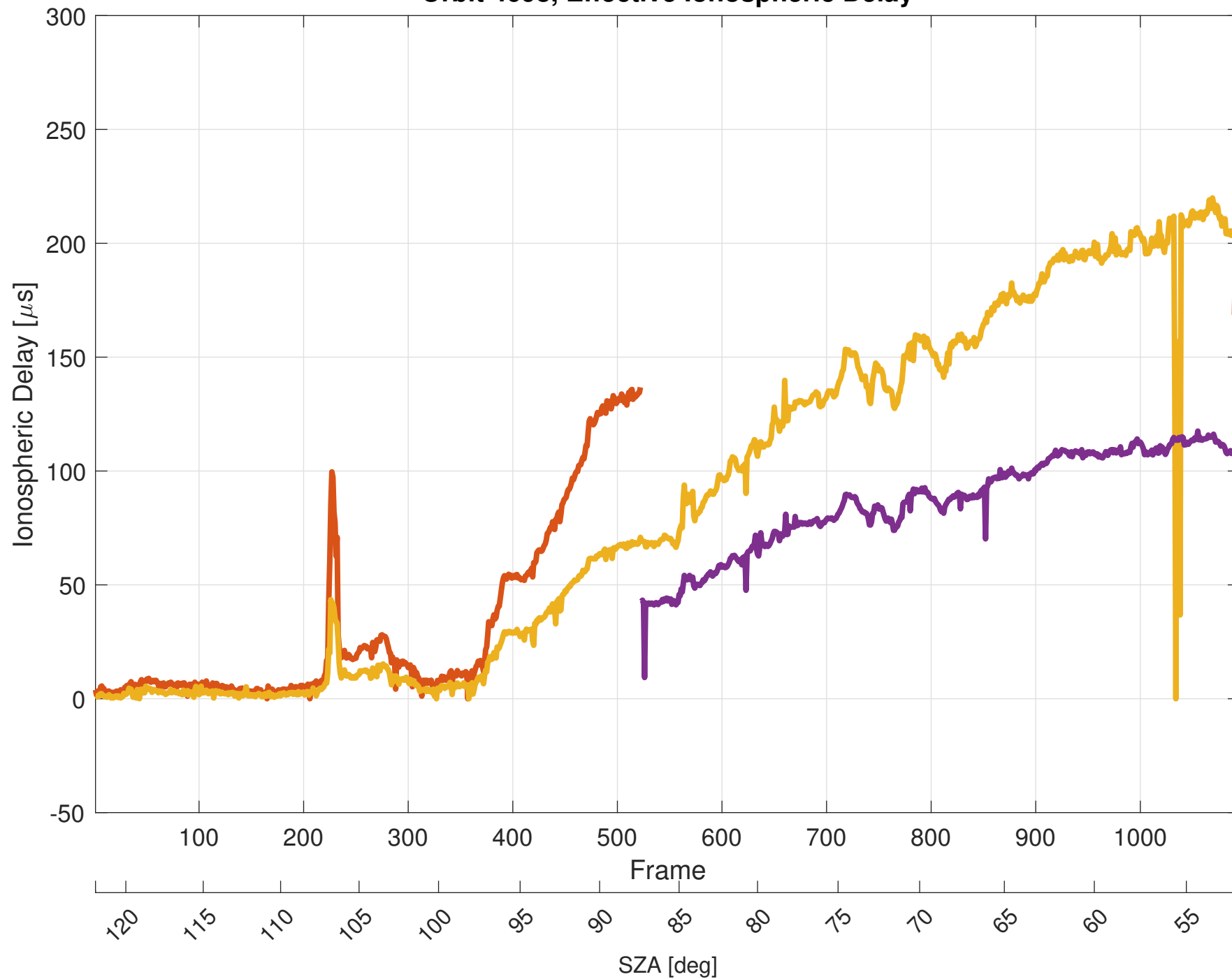
Orbit 4698, Effective Ionospheric Delay
