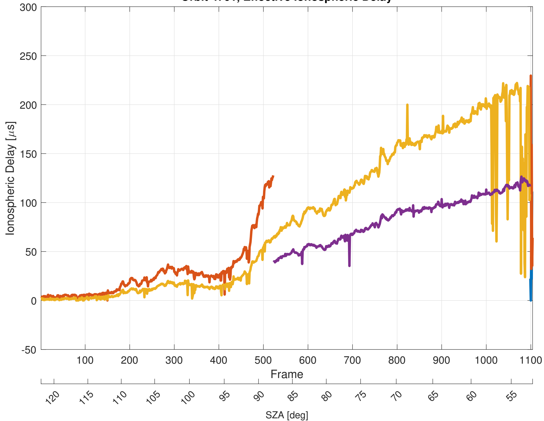
Orbit 4701, Effective Ionospheric Delay
