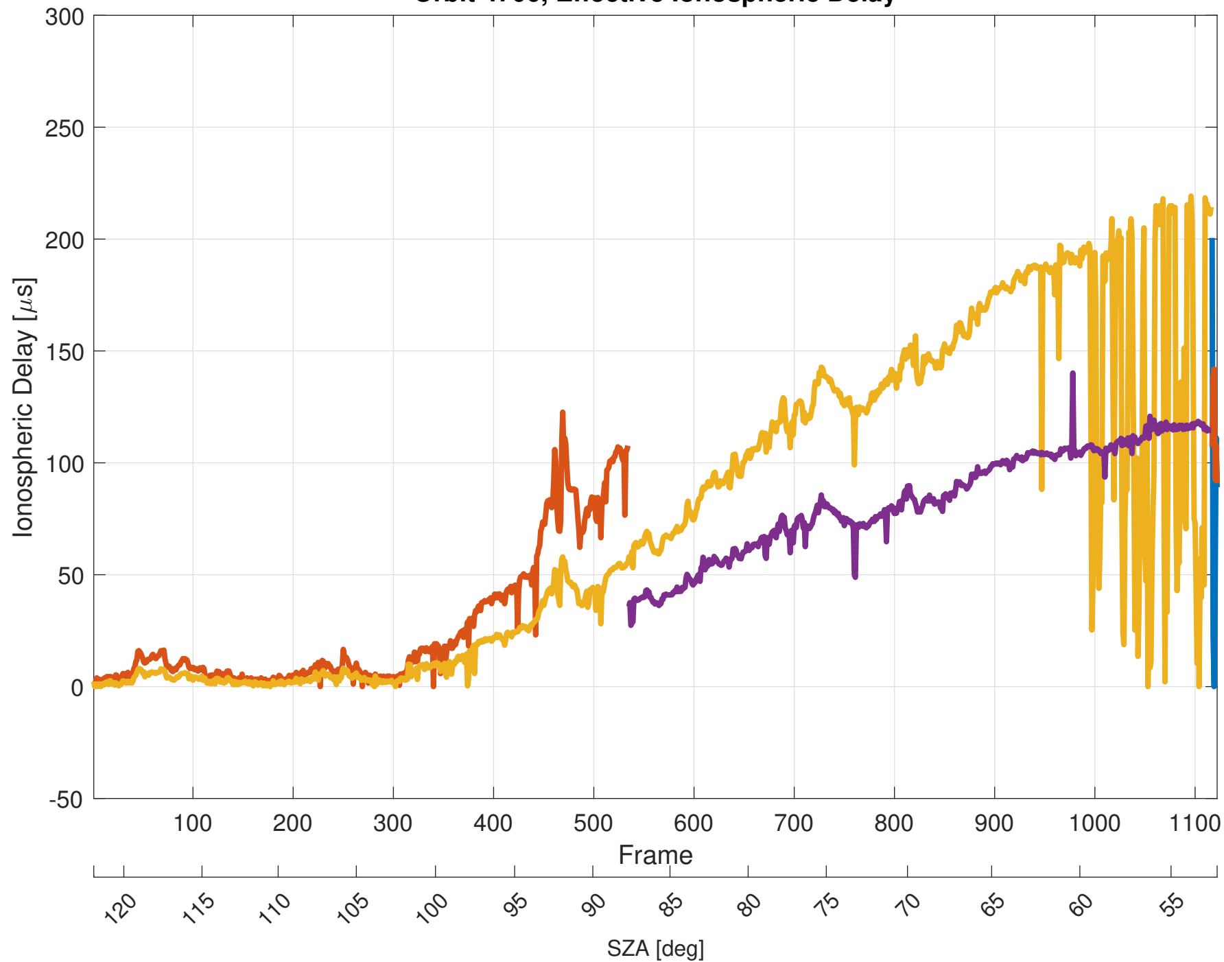
Orbit 4706, Effective Ionospheric Delay
