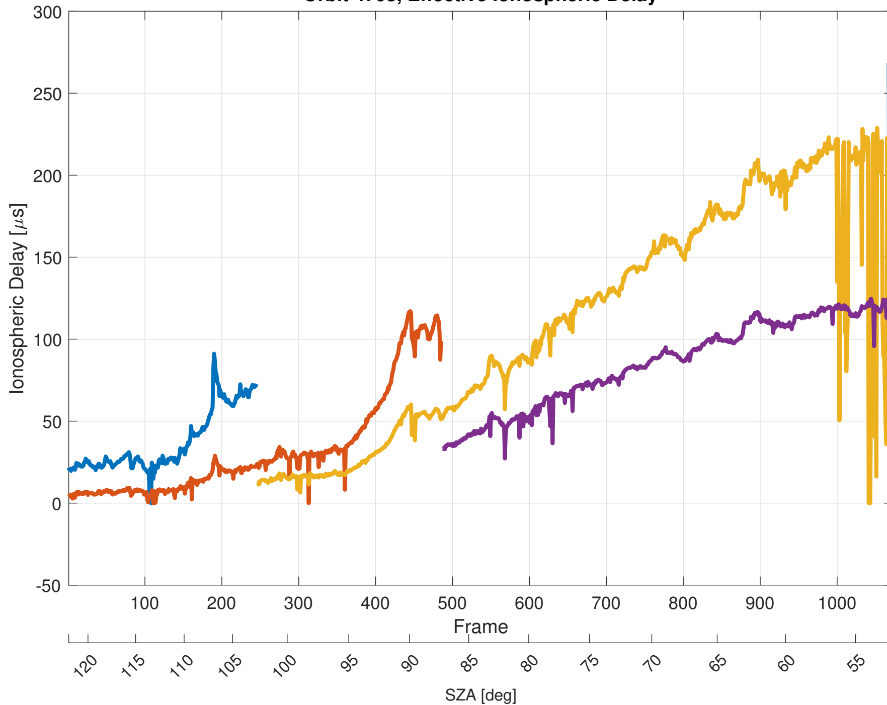
Orbit 4708, Effective Ionospheric Delay
