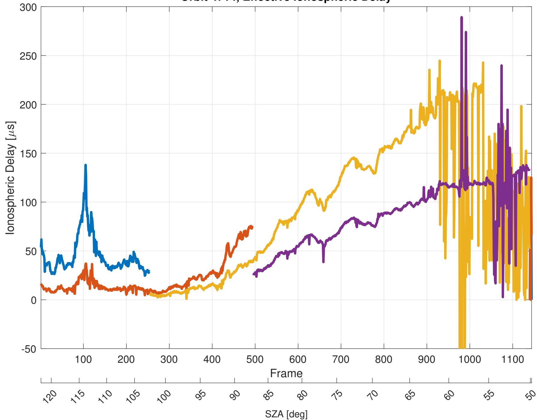
Orbit 4714, Effective Ionospheric Delay
