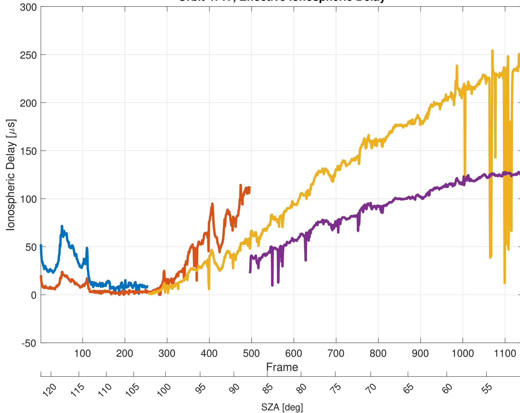
Orbit 4717, Effective Ionospheric Delay
