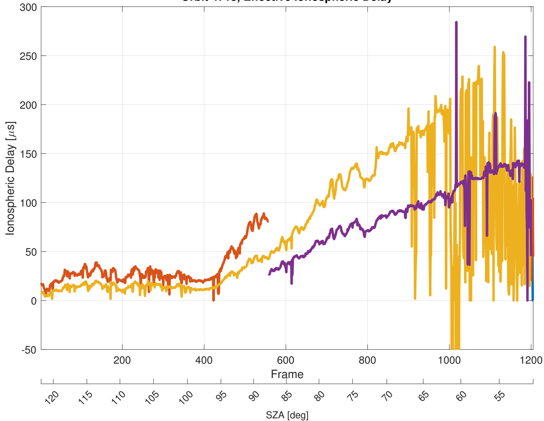
Orbit 4718, Effective Ionospheric Delay
