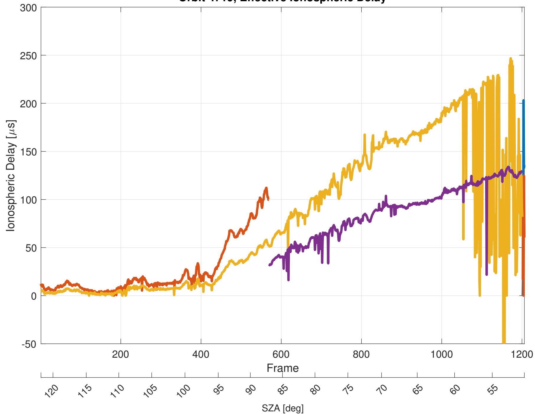
Orbit 4719, Effective Ionospheric Delay
