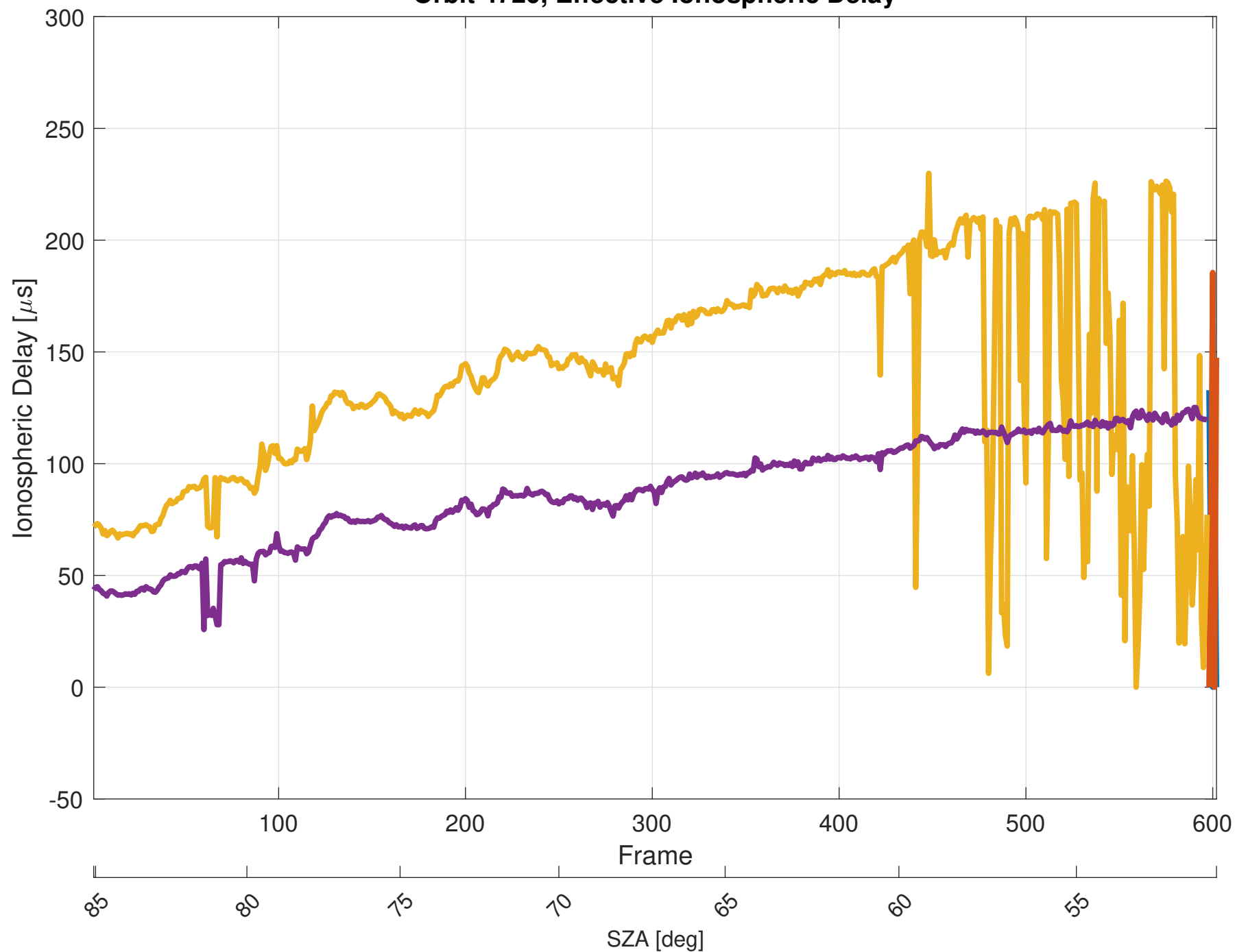
Orbit 4720, Effective Ionospheric Delay
