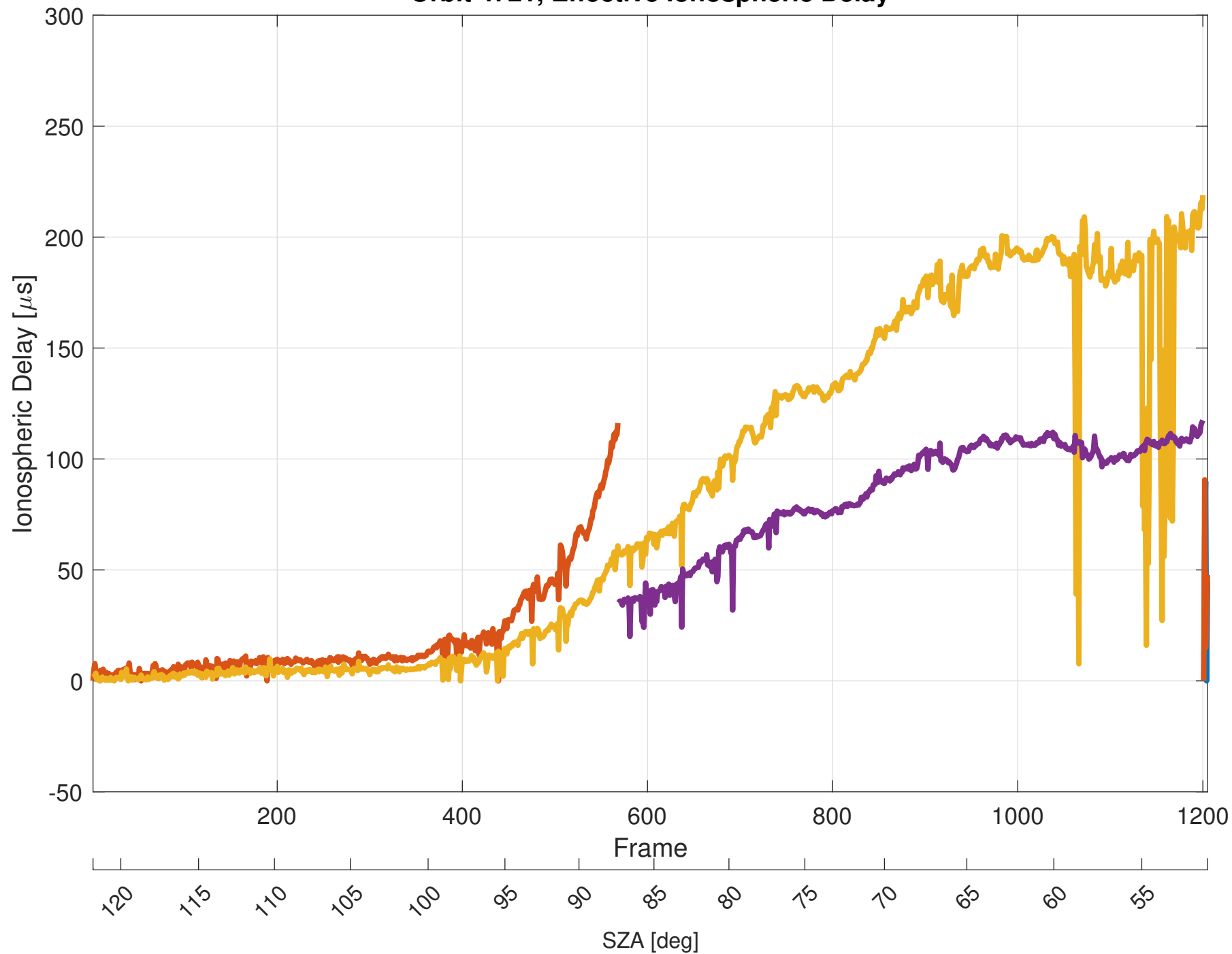
Orbit 4721, Effective Ionospheric Delay
