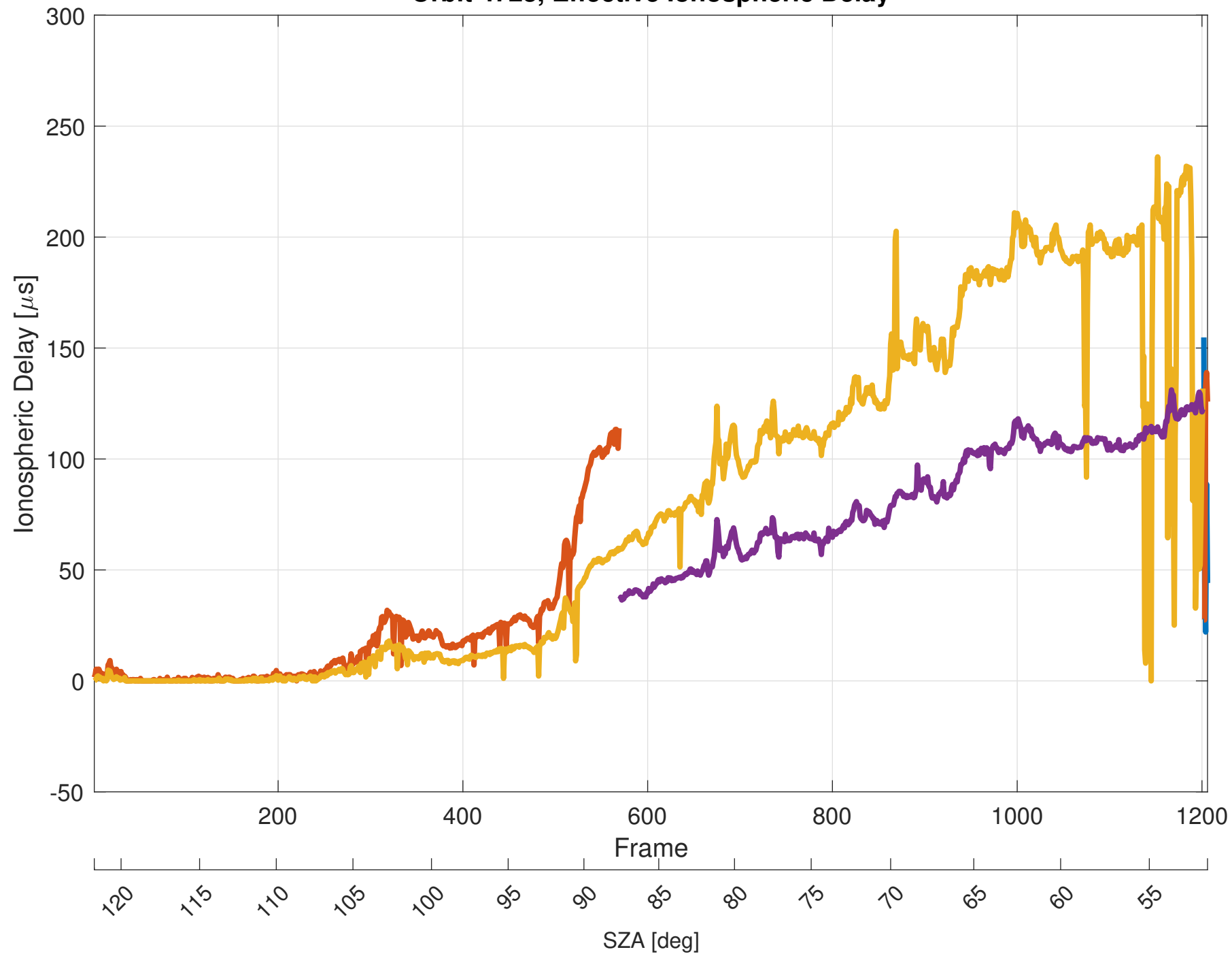
Orbit 4723, Effective Ionospheric Delay
