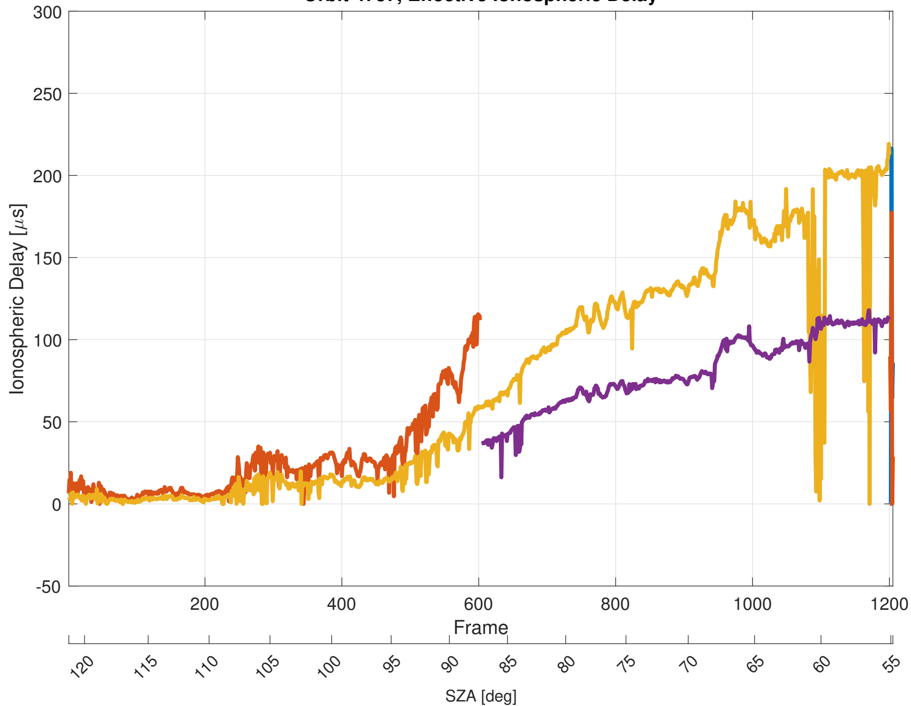
Orbit 4737, Effective Ionospheric Delay
