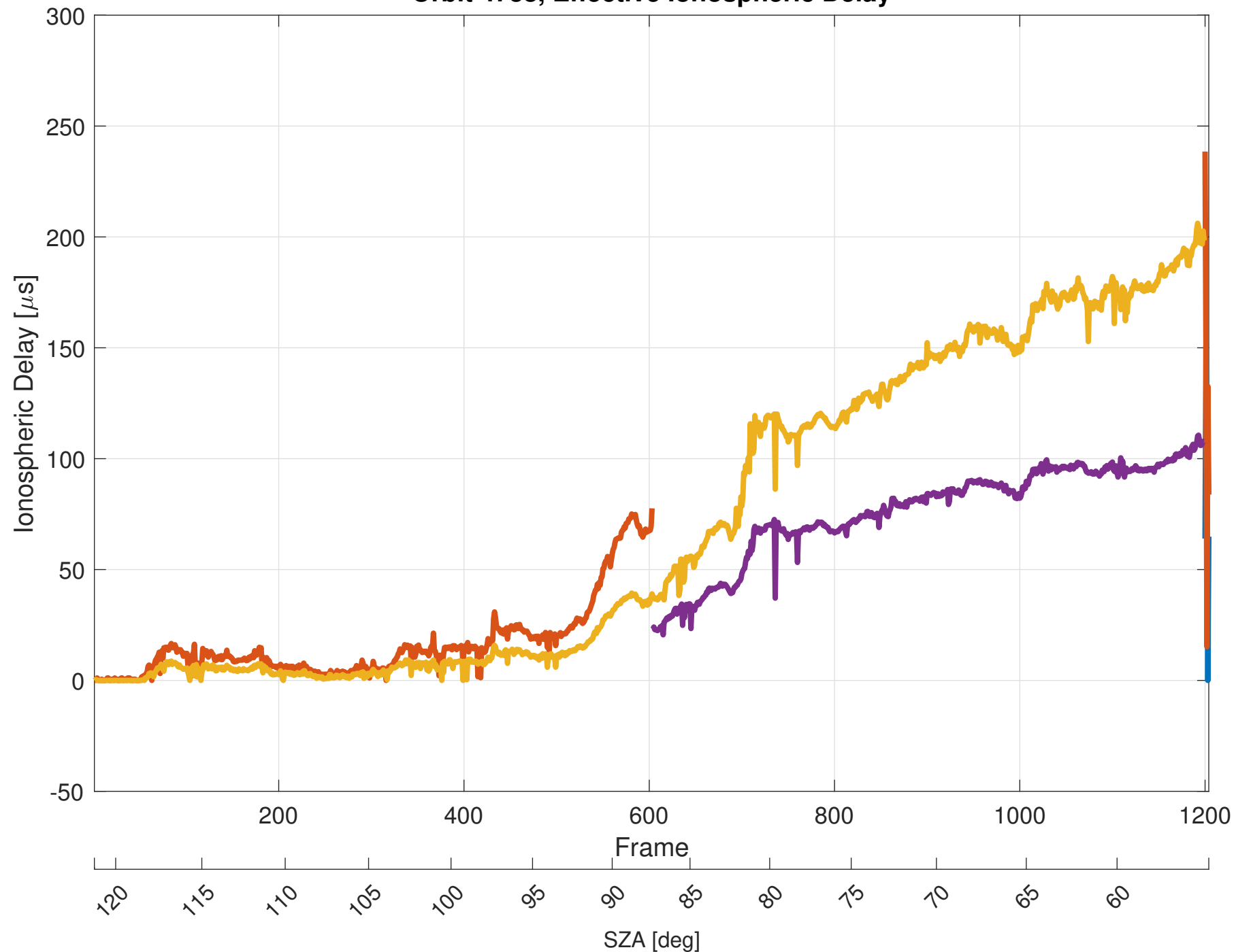
Orbit 4738, Effective Ionospheric Delay
