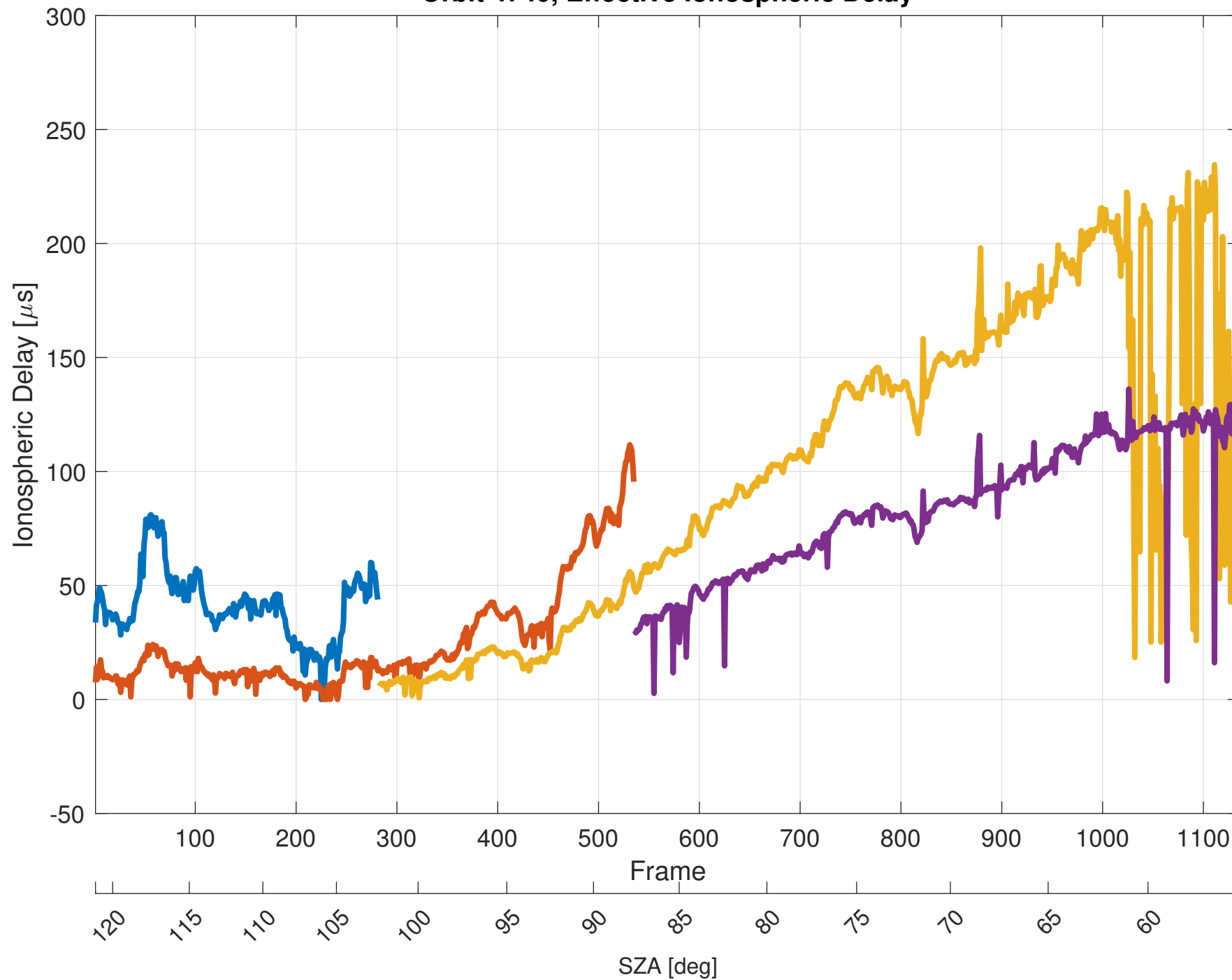
Orbit 4740, Effective Ionospheric Delay
