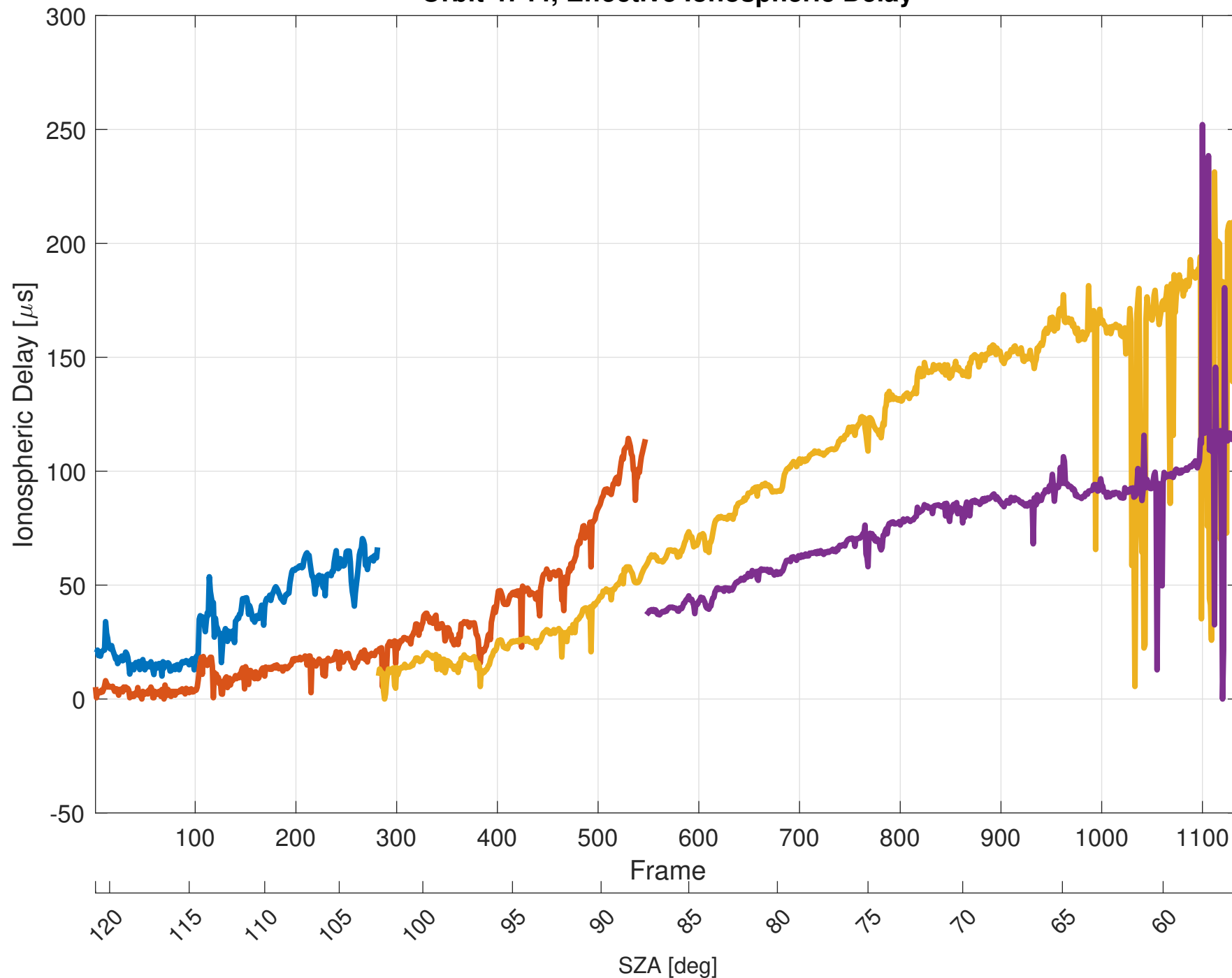
Orbit 4744, Effective Ionospheric Delay
