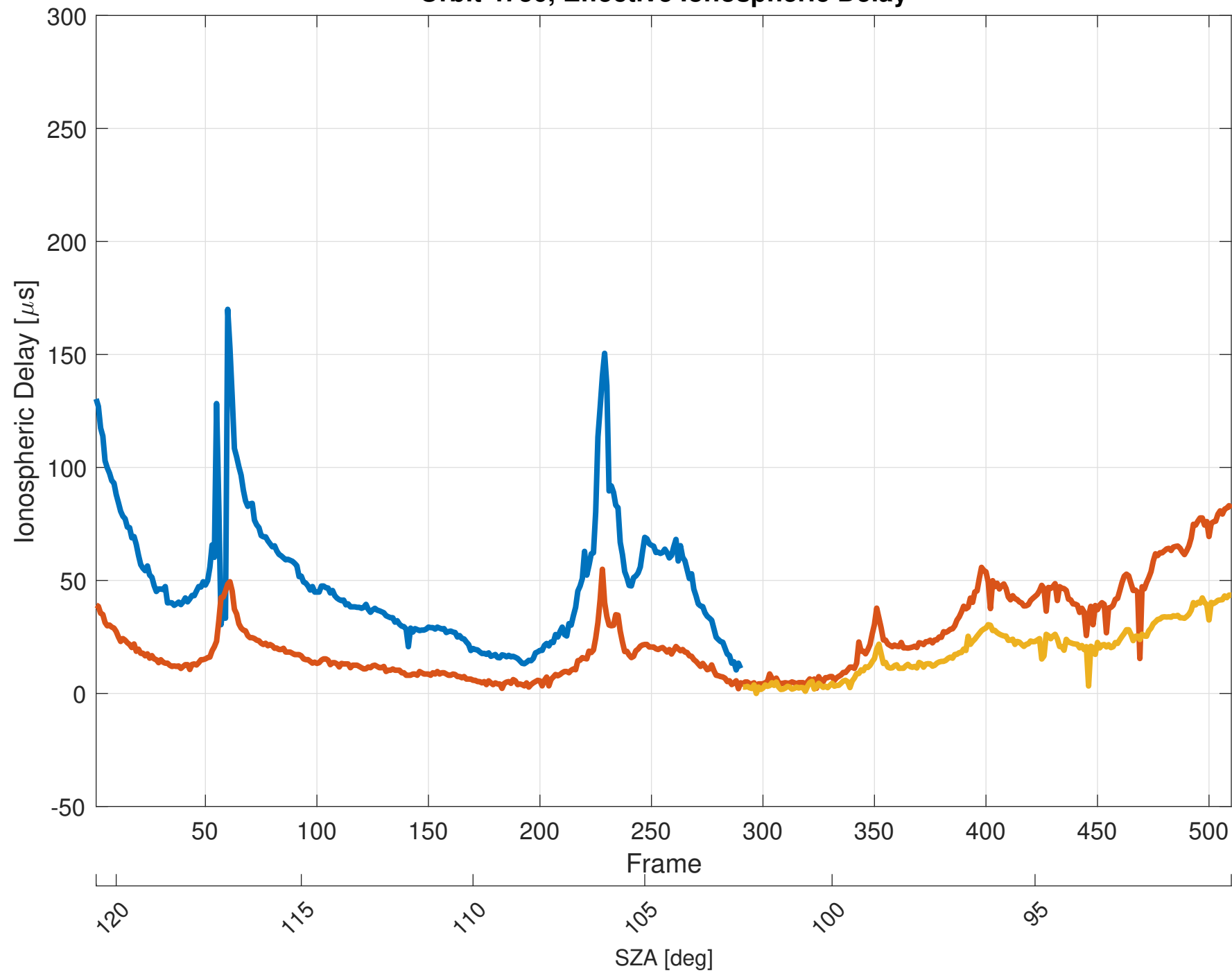
Orbit 4750, Effective Ionospheric Delay
