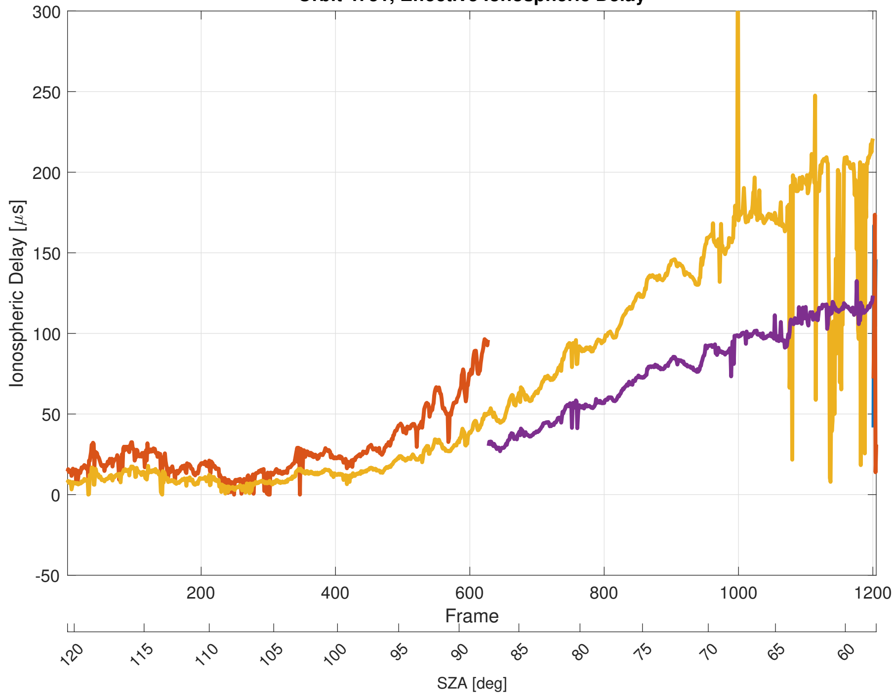
Orbit 4751, Effective Ionospheric Delay
