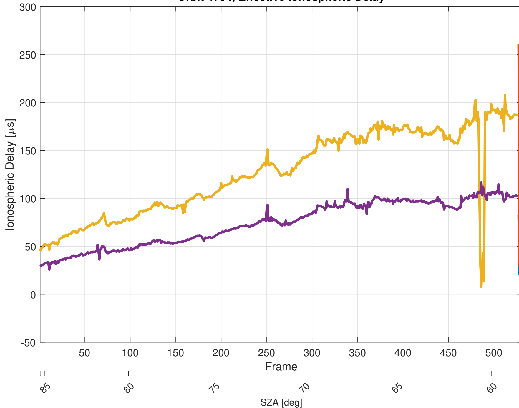
Orbit 4754, Effective Ionospheric Delay
