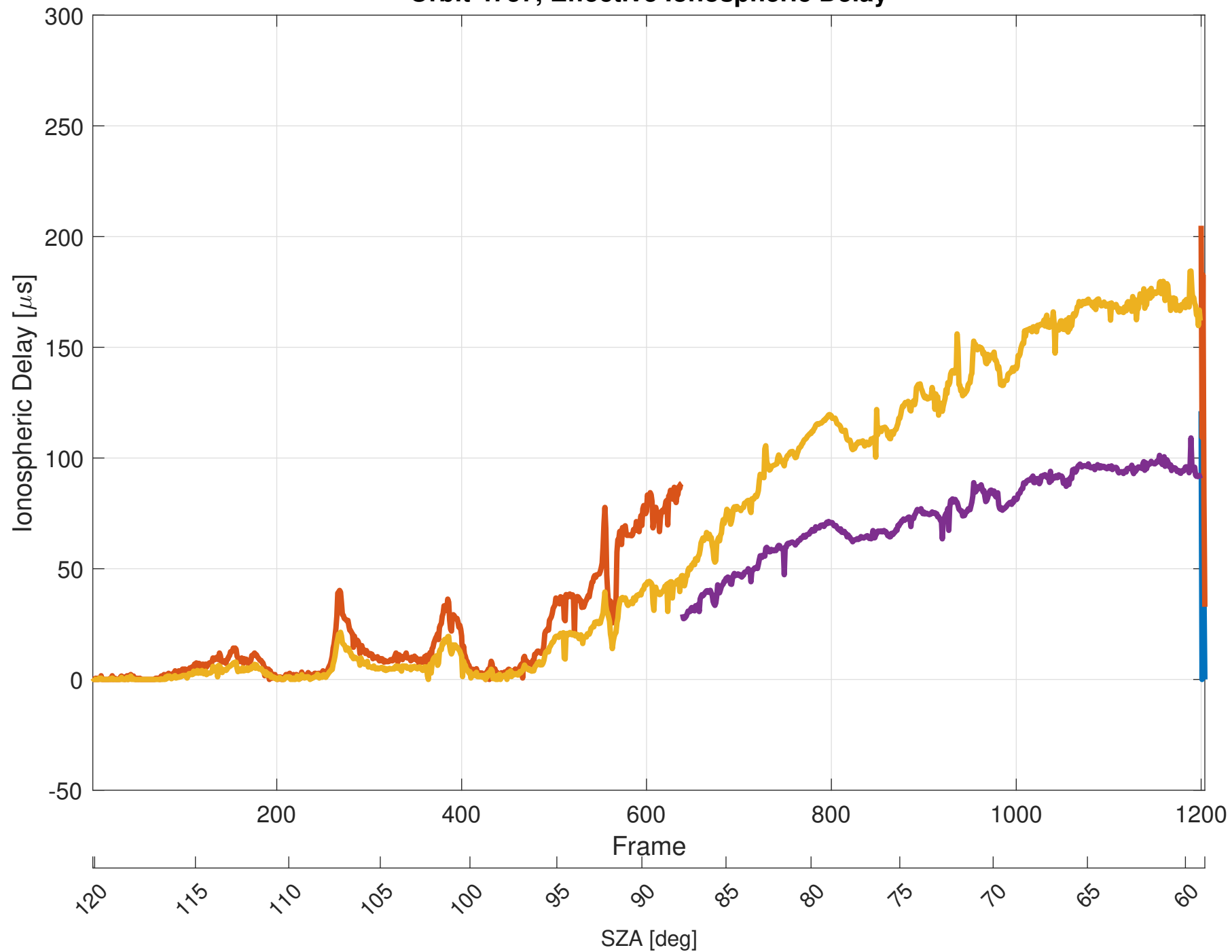
Orbit 4757, Effective Ionospheric Delay
