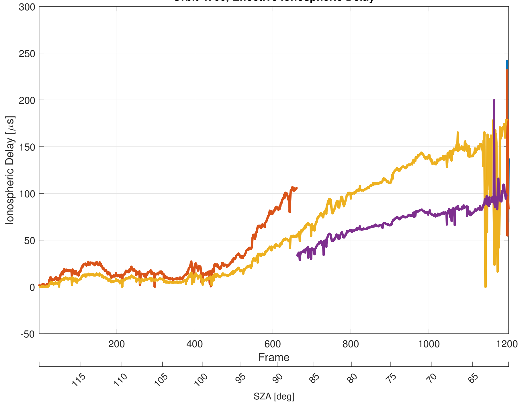
Orbit 4766, Effective Ionospheric Delay
