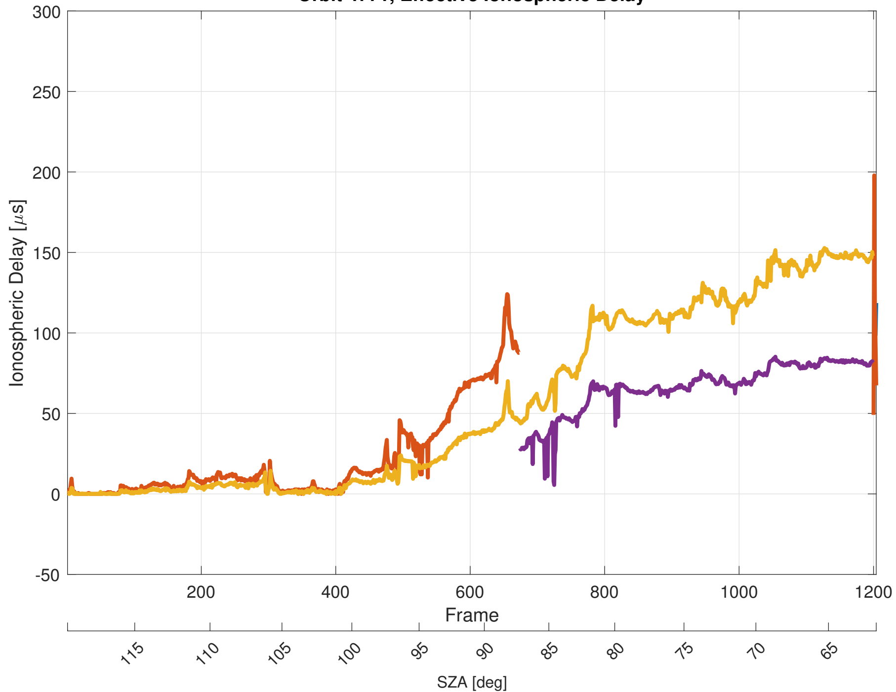
Orbit 4771, Effective Ionospheric Delay
