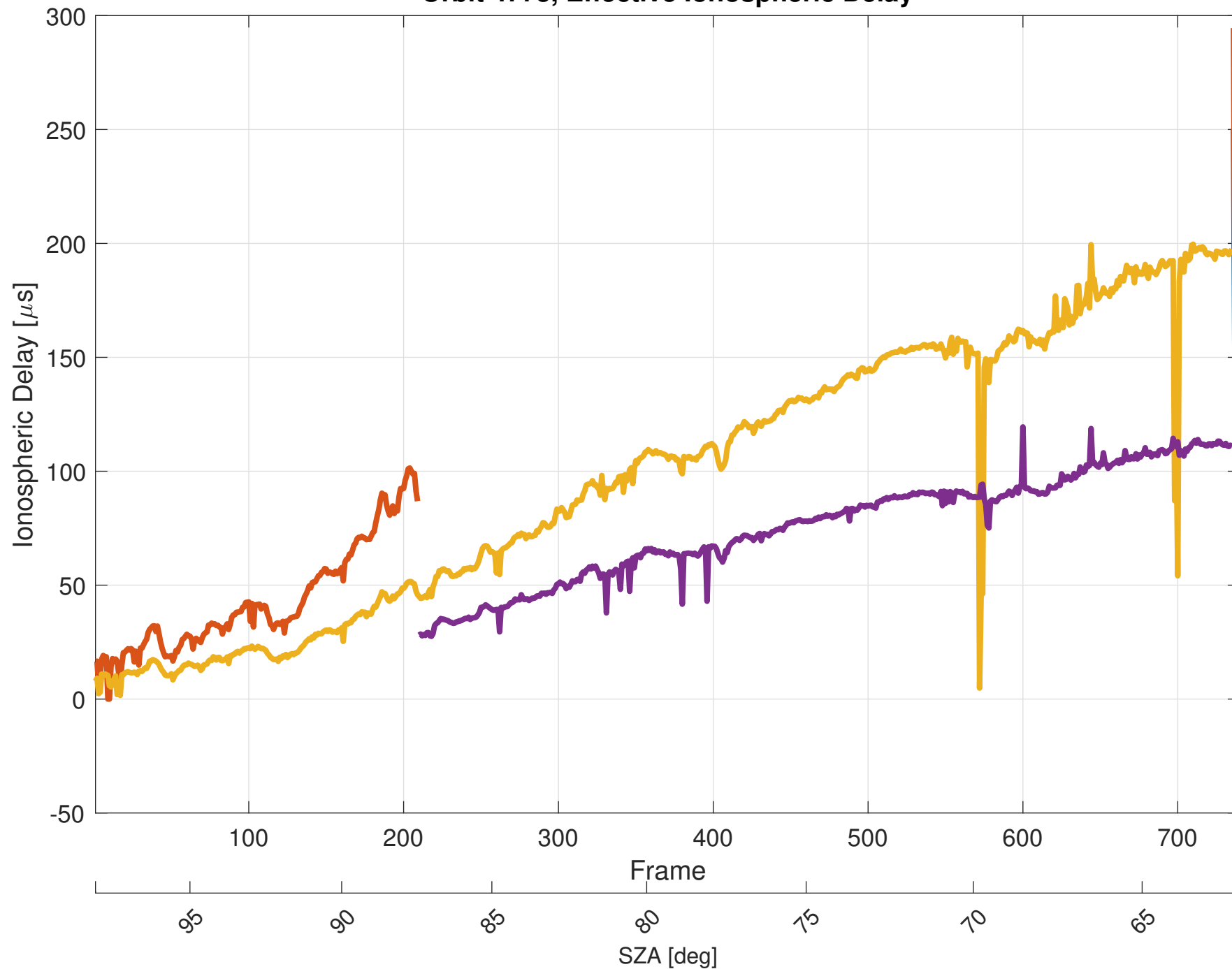
Orbit 4773, Effective Ionospheric Delay
