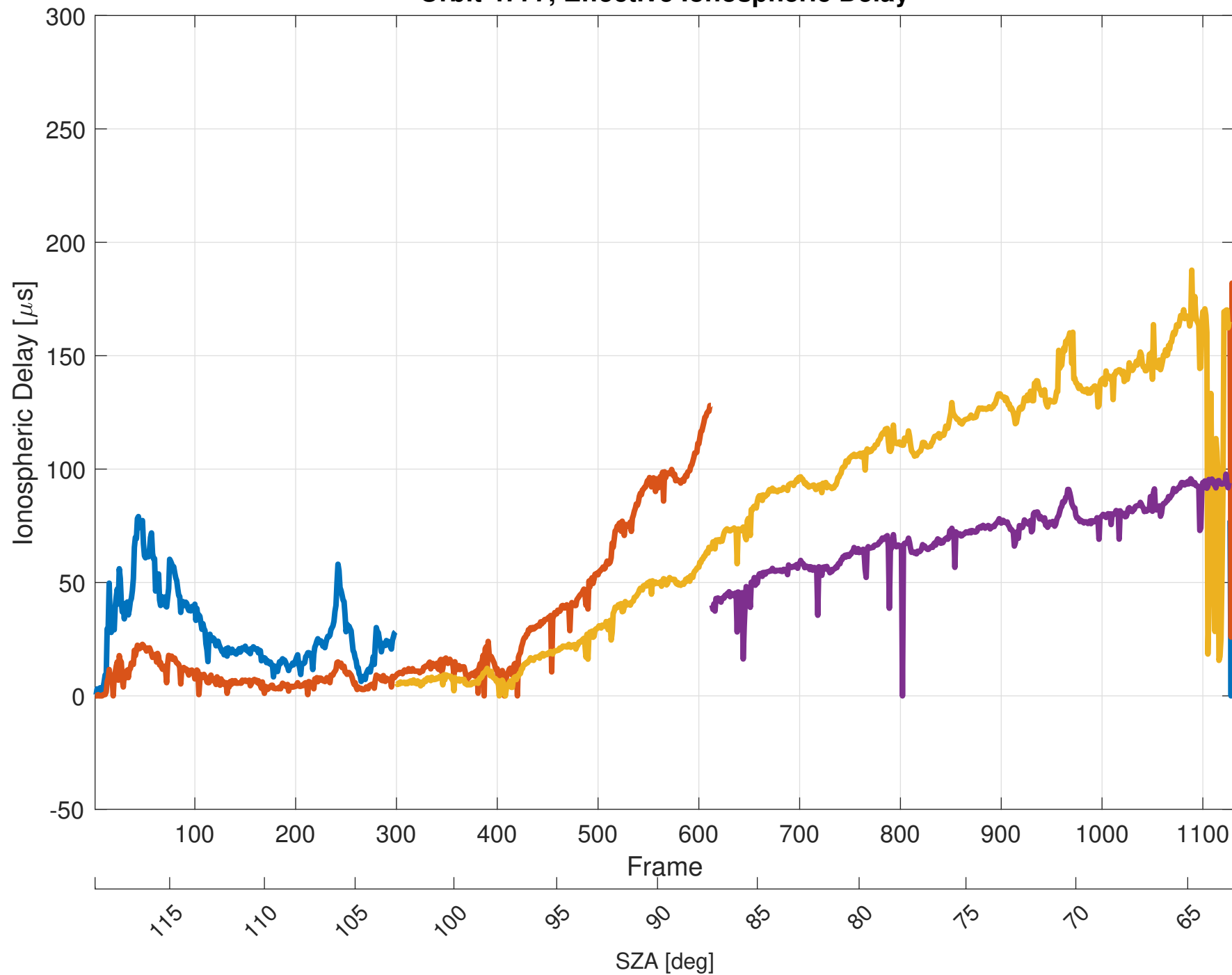
Orbit 4777, Effective Ionospheric Delay
