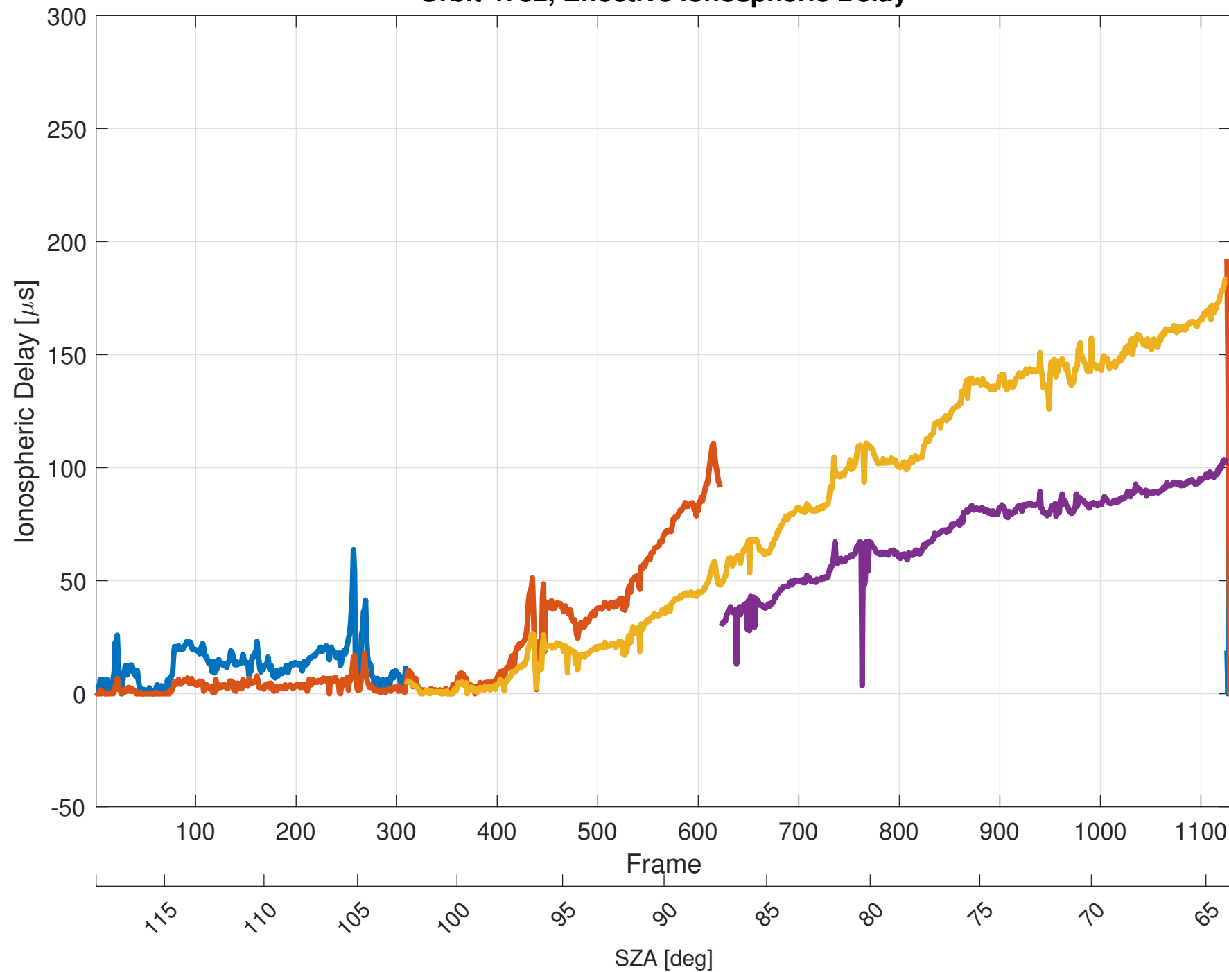
Orbit 4782, Effective Ionospheric Delay
