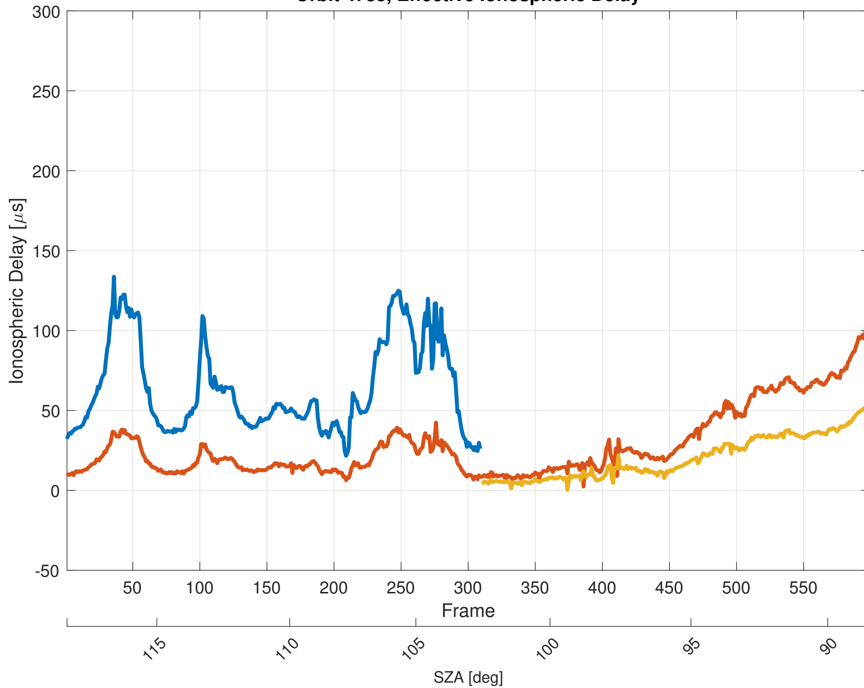
Orbit 4783, Effective Ionospheric Delay
