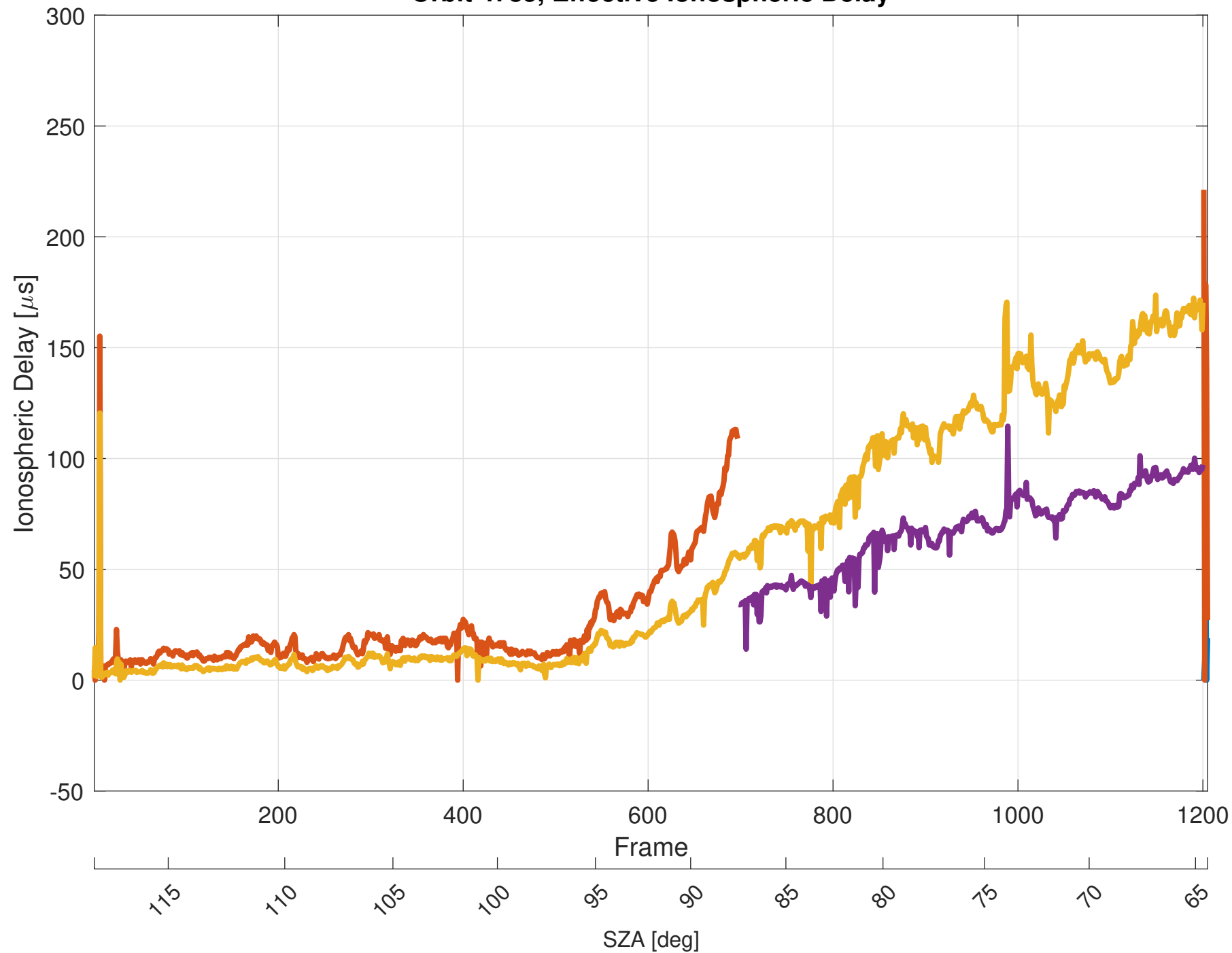
Orbit 4785, Effective Ionospheric Delay
