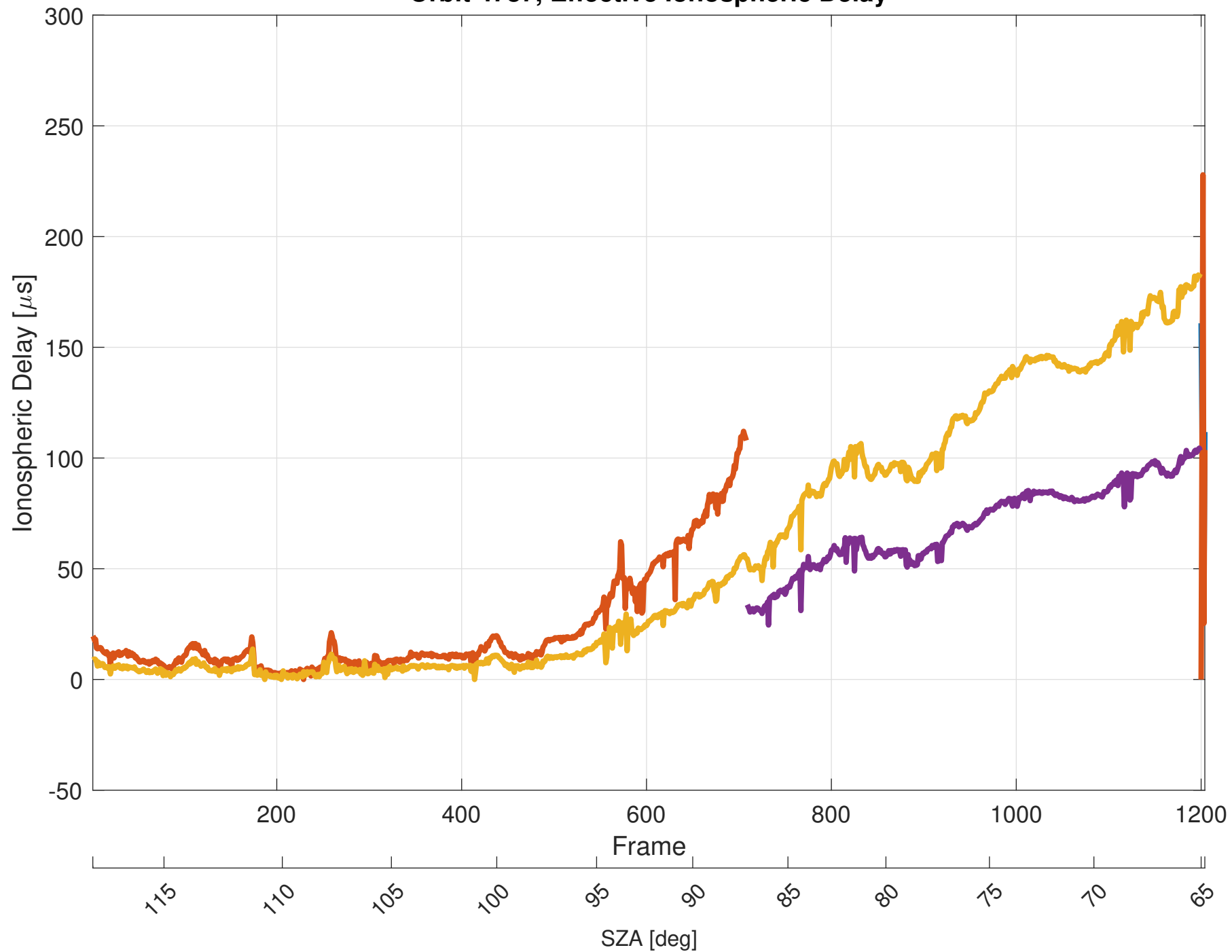
Orbit 4787, Effective Ionospheric Delay
