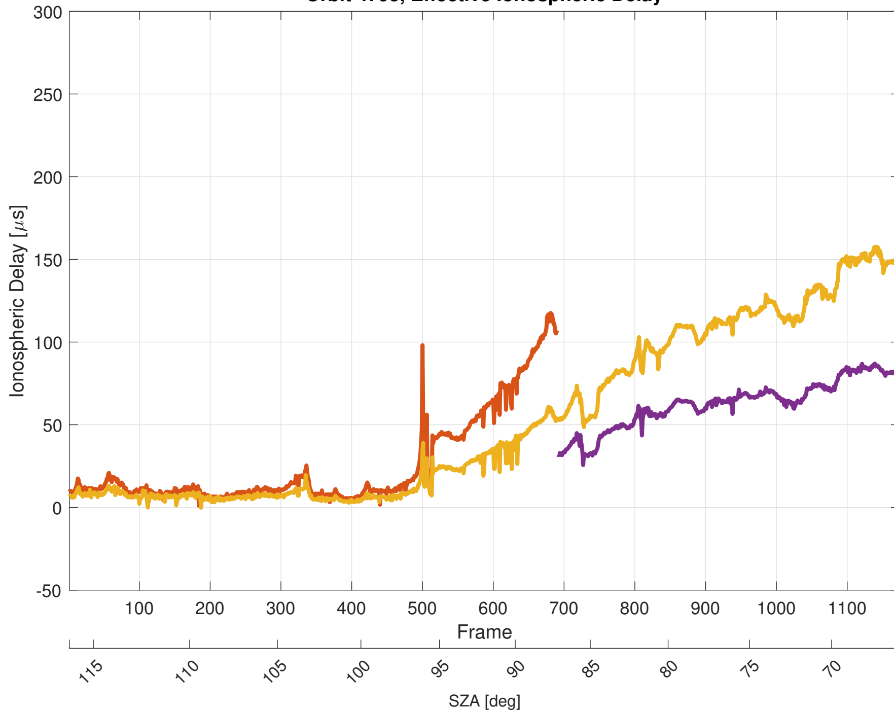
Orbit 4793, Effective Ionospheric Delay
