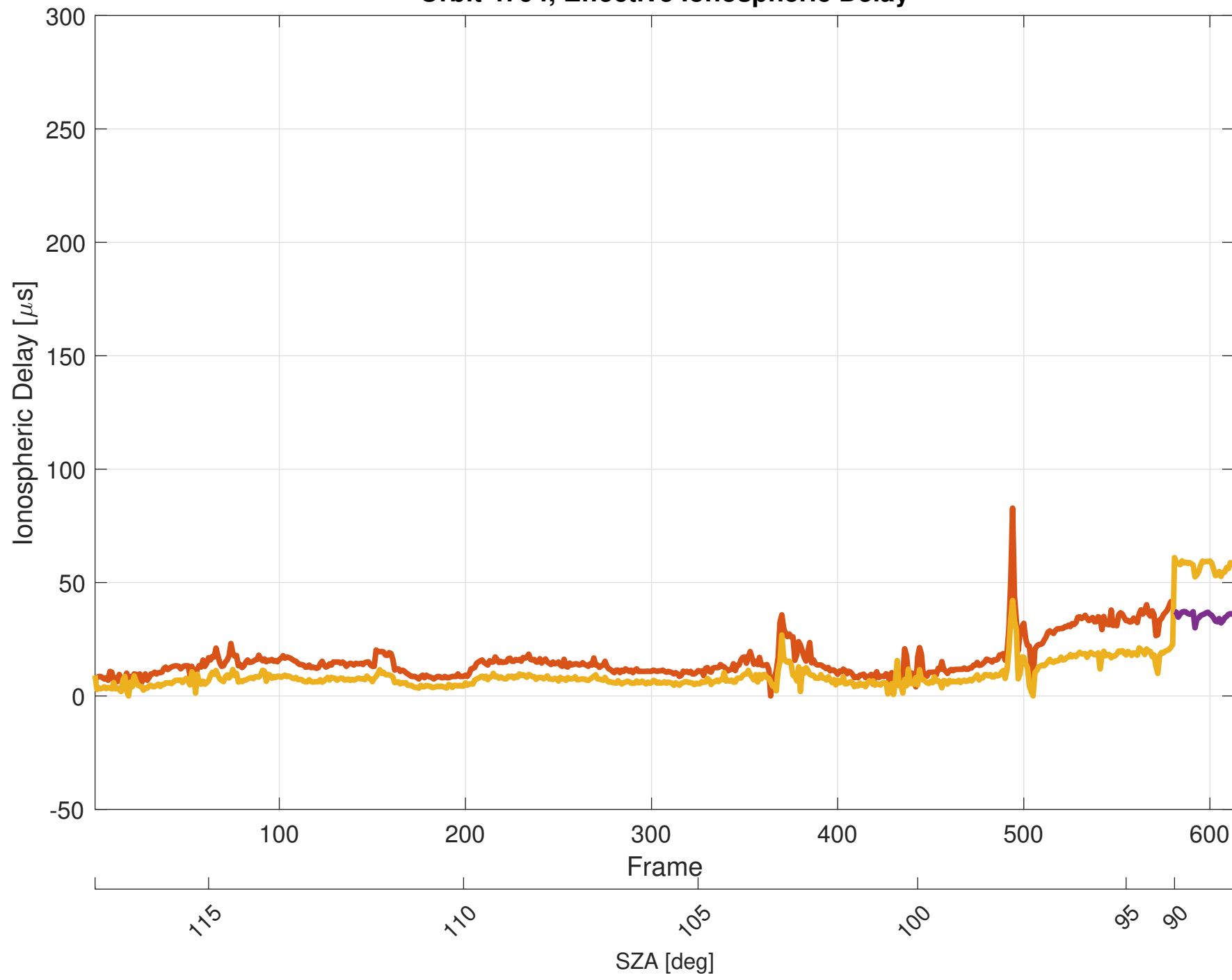
Orbit 4794, Effective Ionospheric Delay
