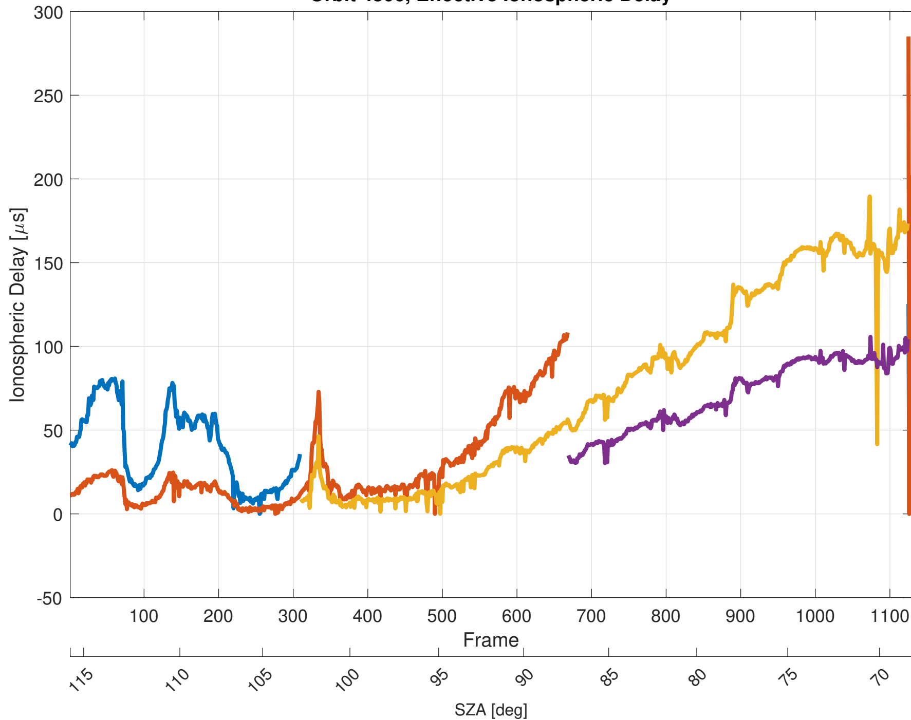
Orbit 4806, Effective Ionospheric Delay
