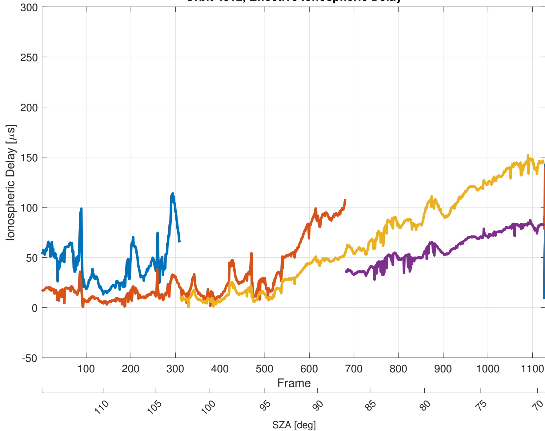
Orbit 4812, Effective Ionospheric Delay
