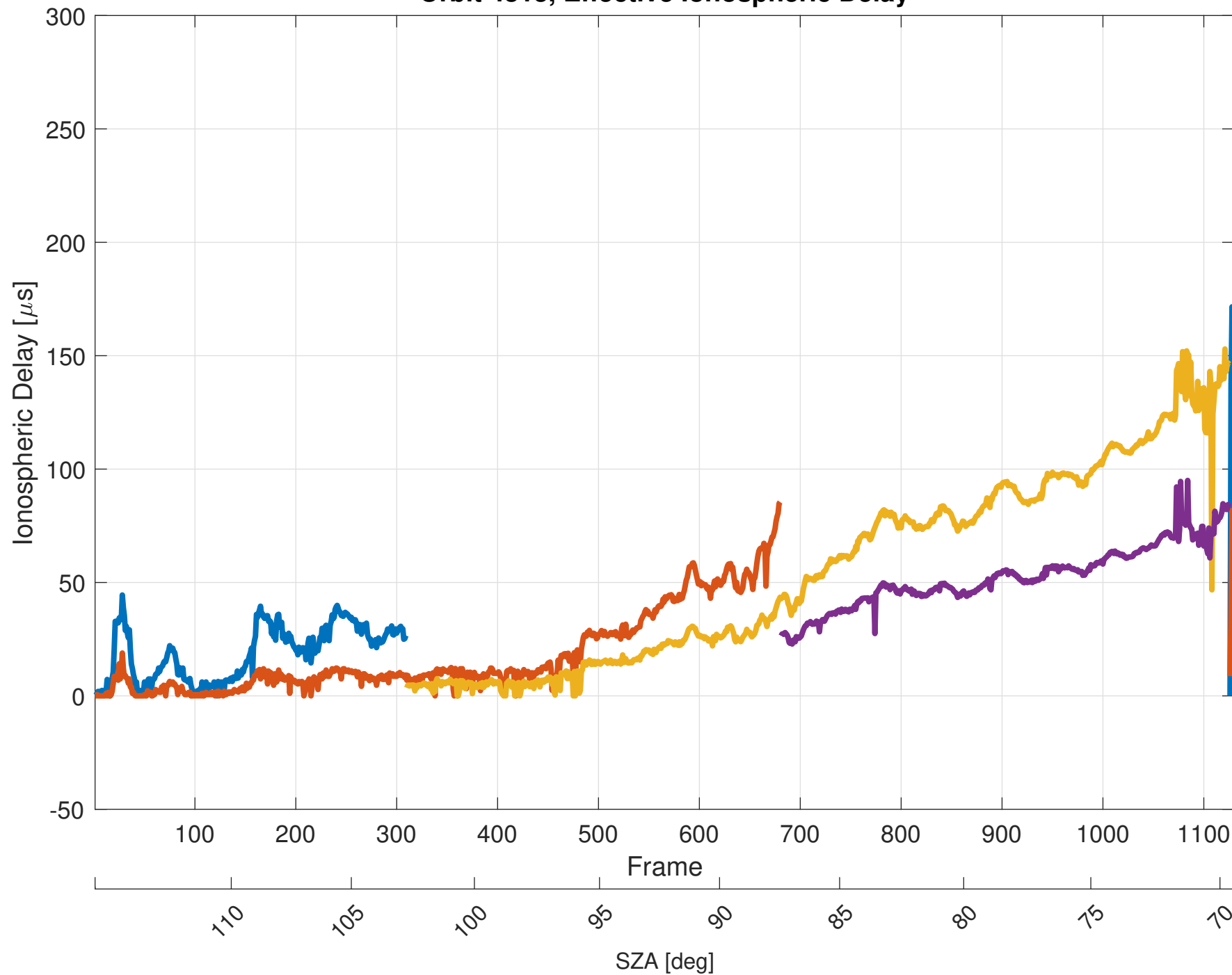
Orbit 4813, Effective Ionospheric Delay
