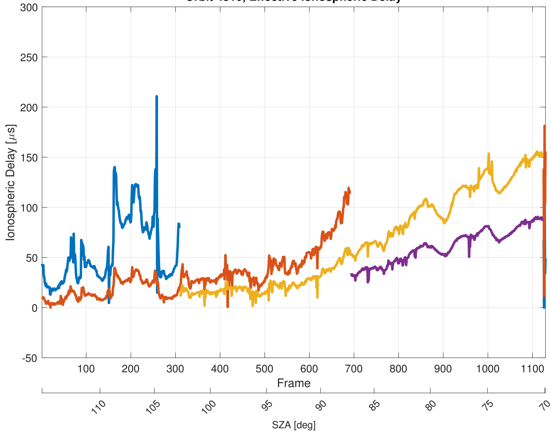
Orbit 4816, Effective Ionospheric Delay
