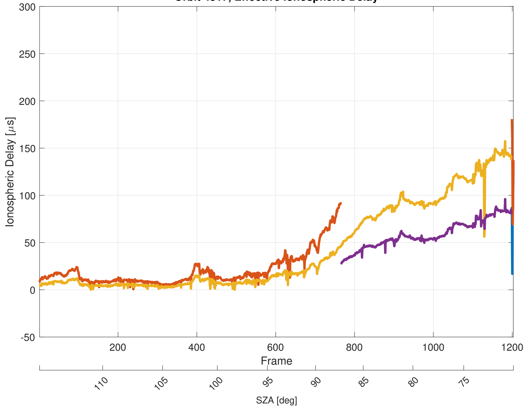
Orbit 4817, Effective Ionospheric Delay
