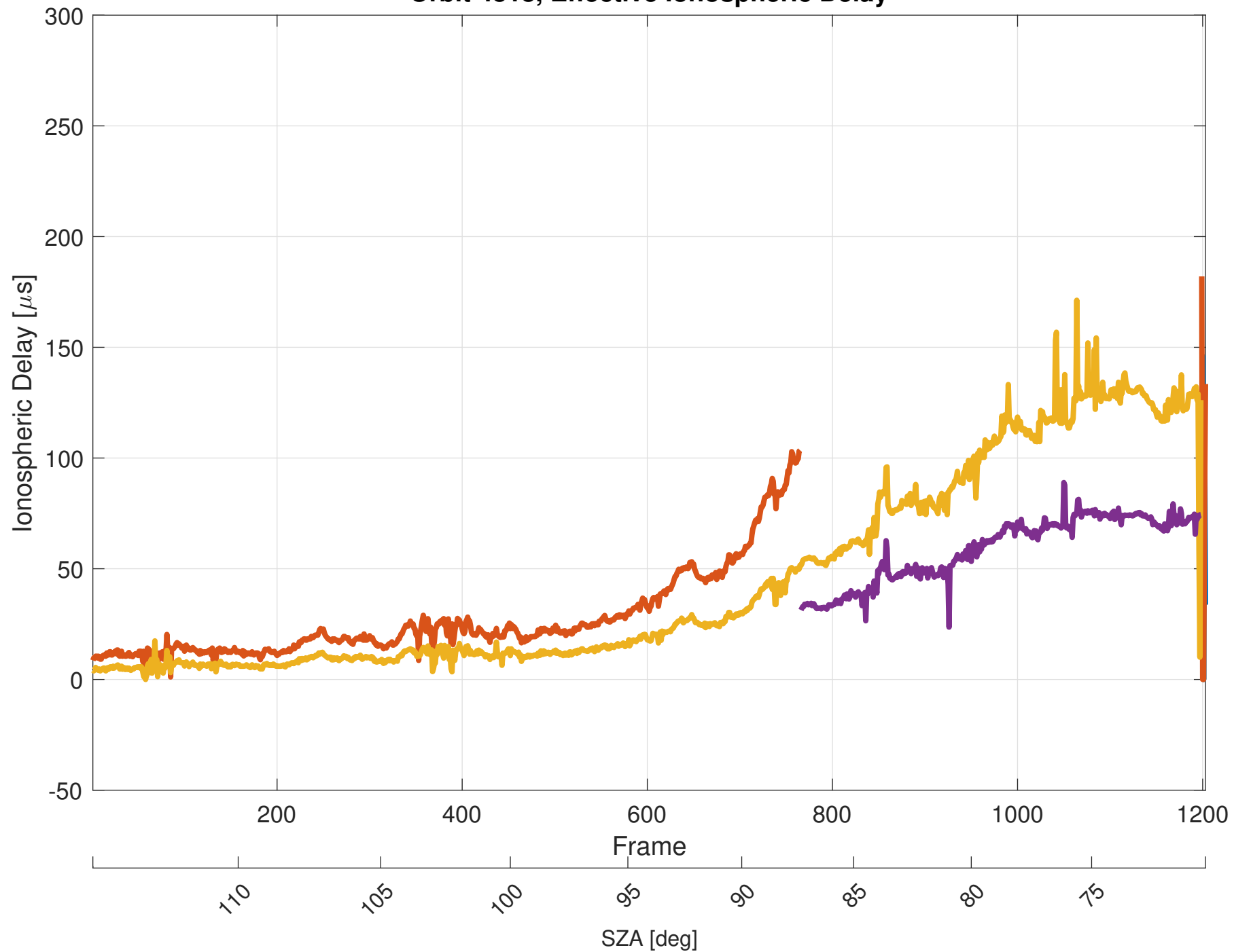
Orbit 4818, Effective Ionospheric Delay
