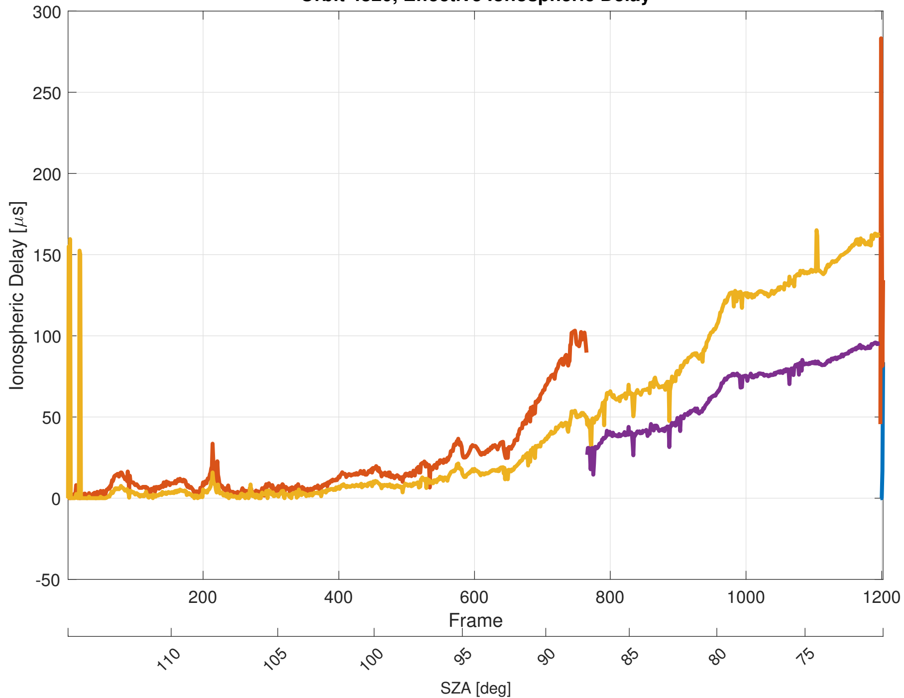
Orbit 4820, Effective Ionospheric Delay
