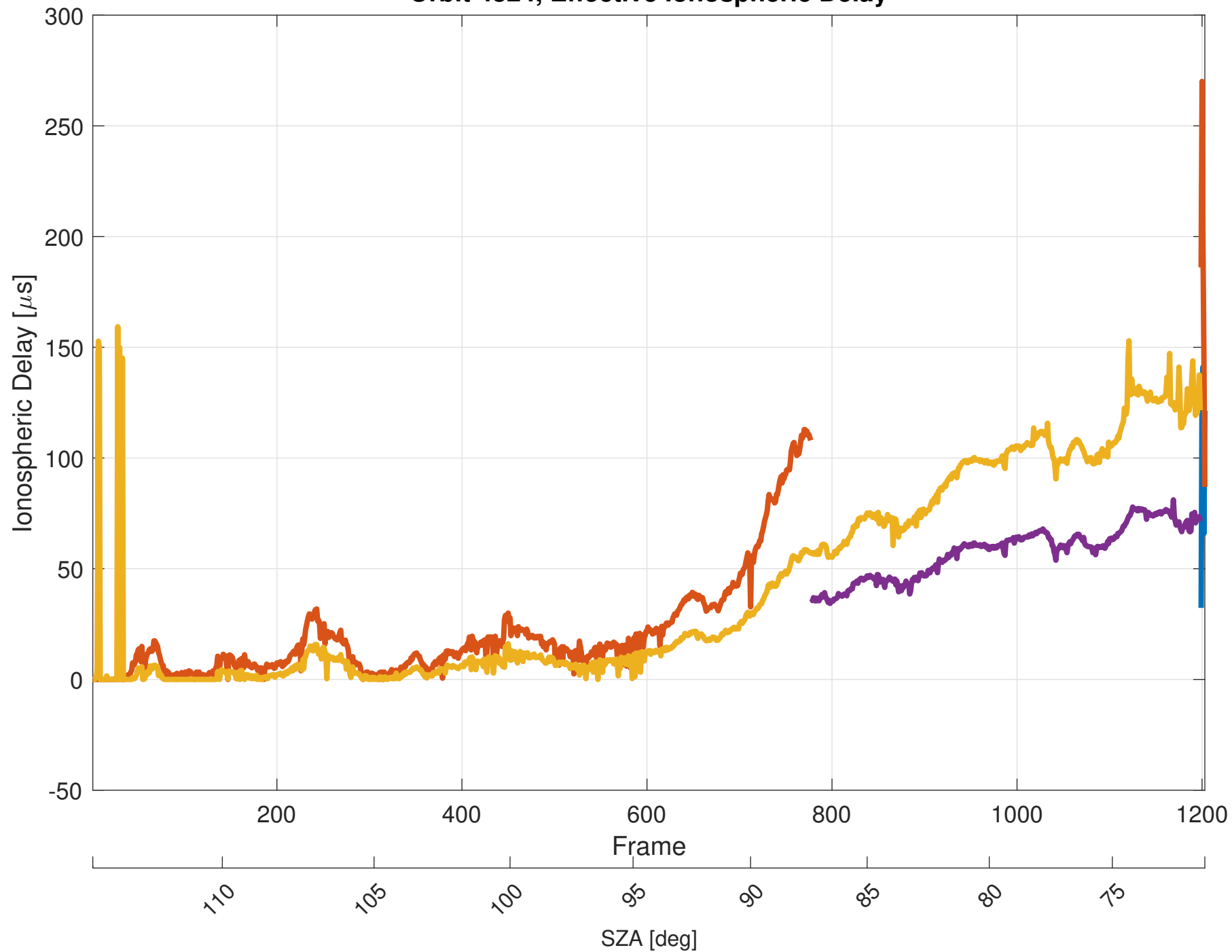
Orbit 4824, Effective Ionospheric Delay
