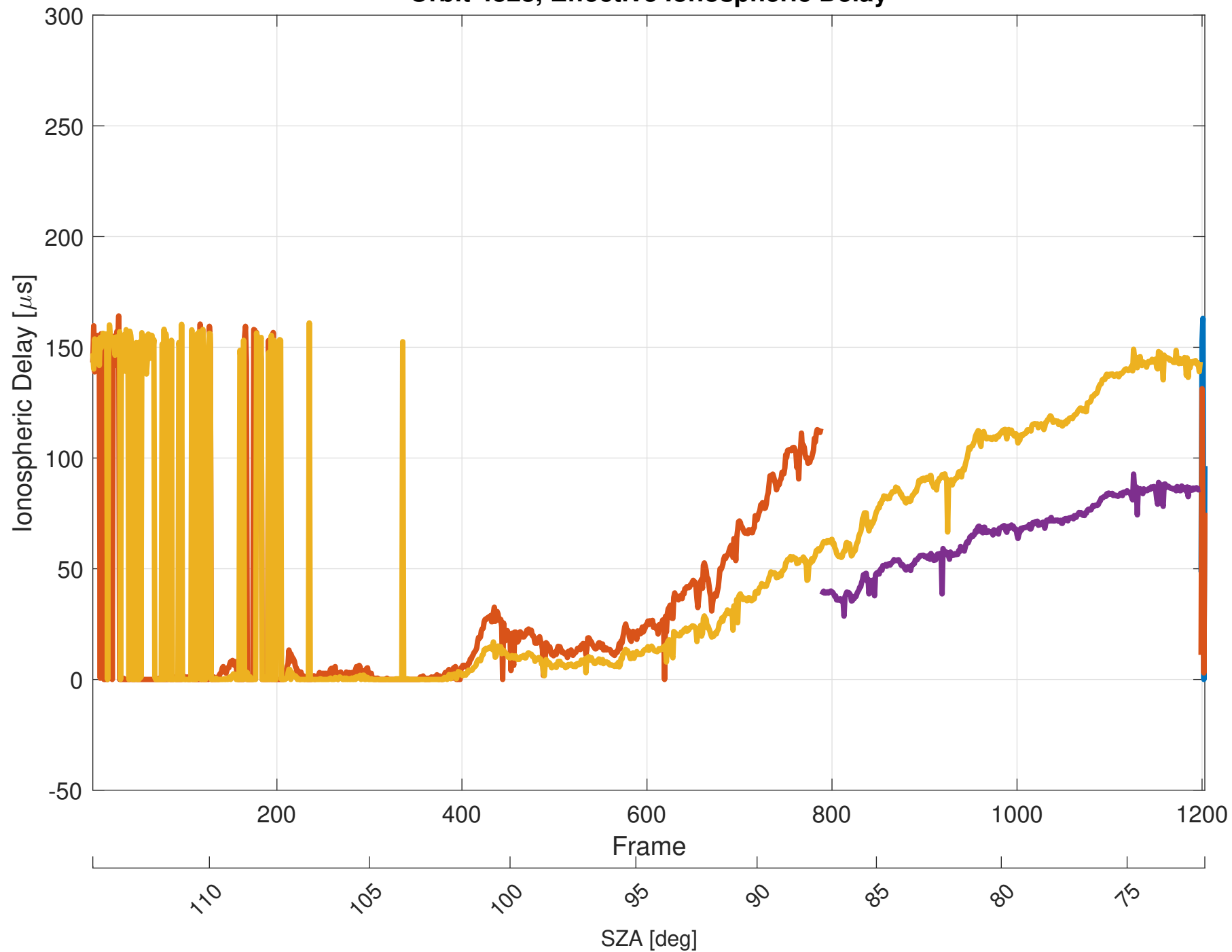
Orbit 4828, Effective Ionospheric Delay
