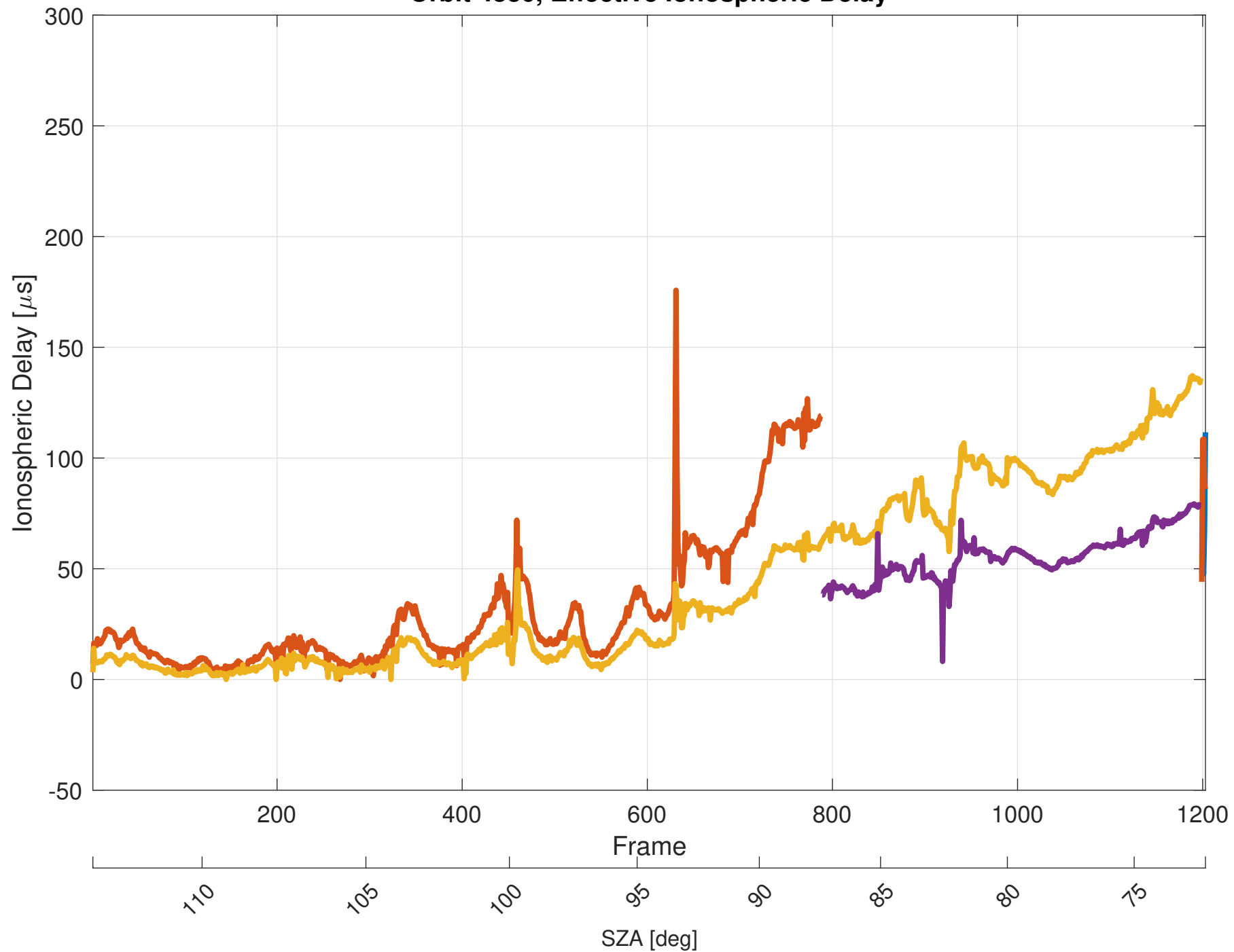
Orbit 4830, Effective Ionospheric Delay
