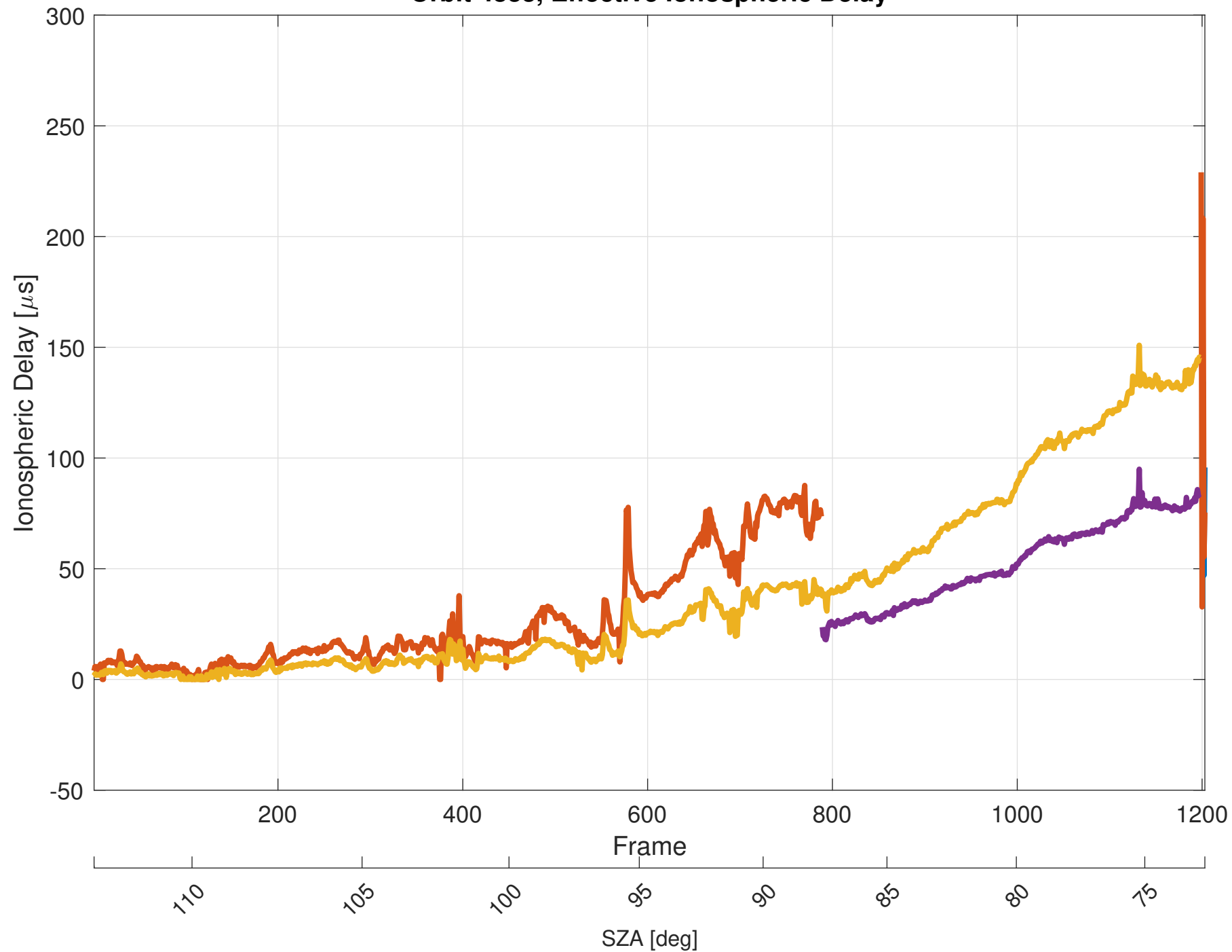
Orbit 4833, Effective Ionospheric Delay
