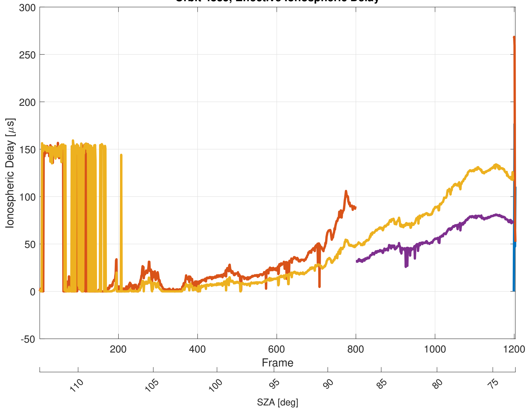
Orbit 4835, Effective Ionospheric Delay
