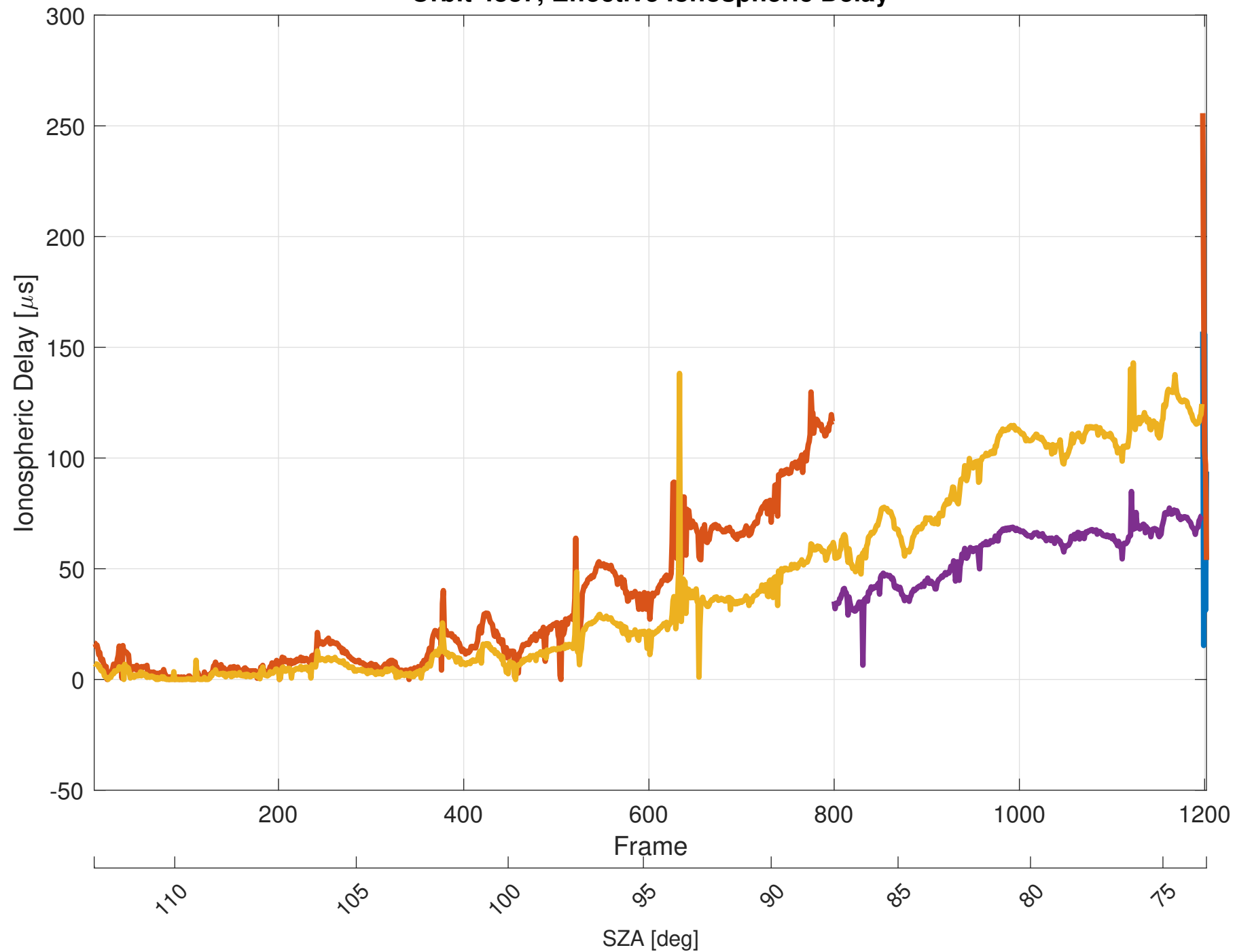
Orbit 4837, Effective Ionospheric Delay
