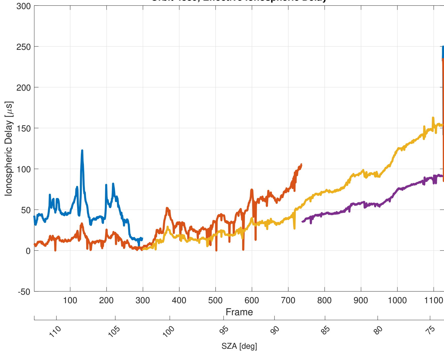
Orbit 4839, Effective Ionospheric Delay
