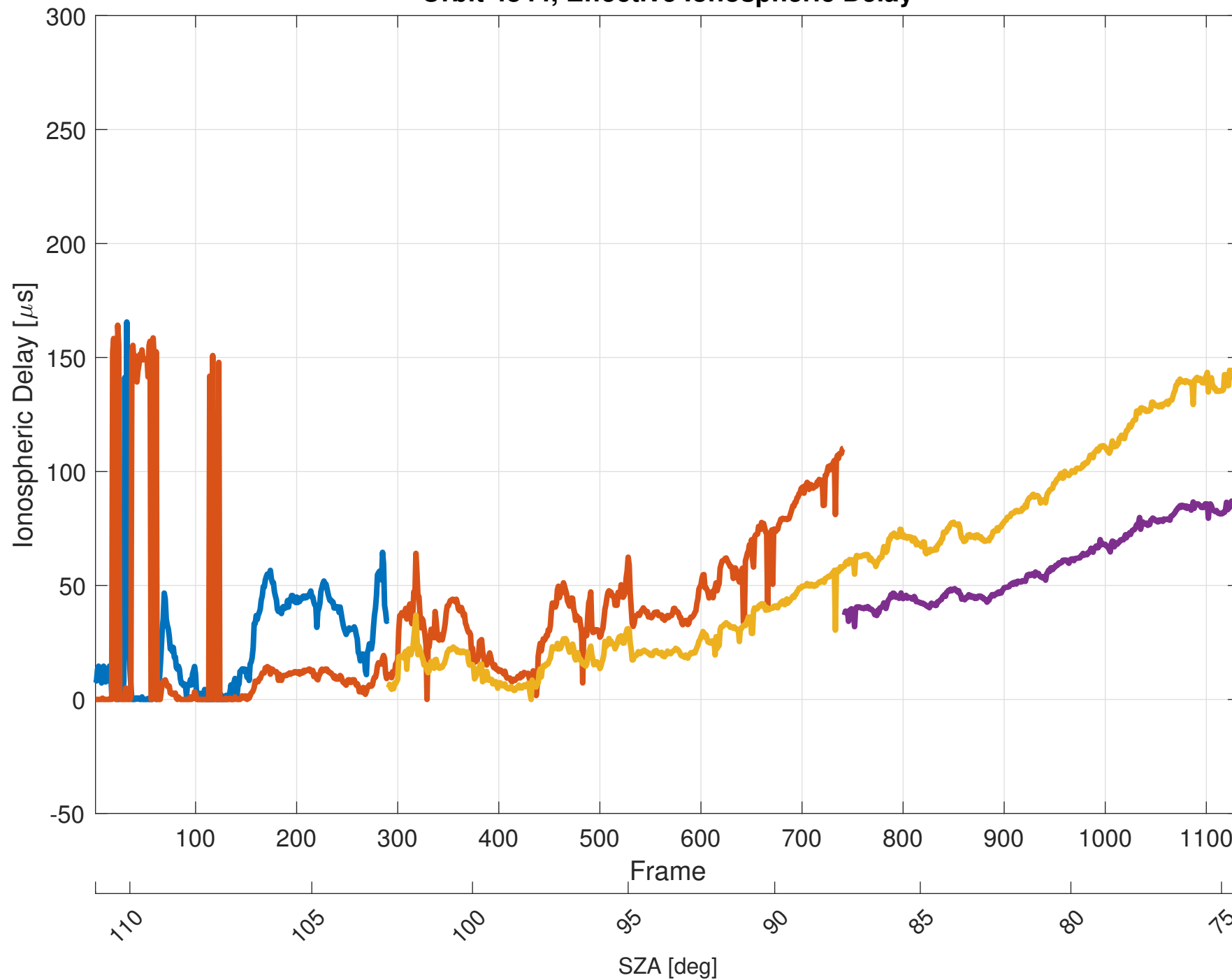
Orbit 4844, Effective Ionospheric Delay
