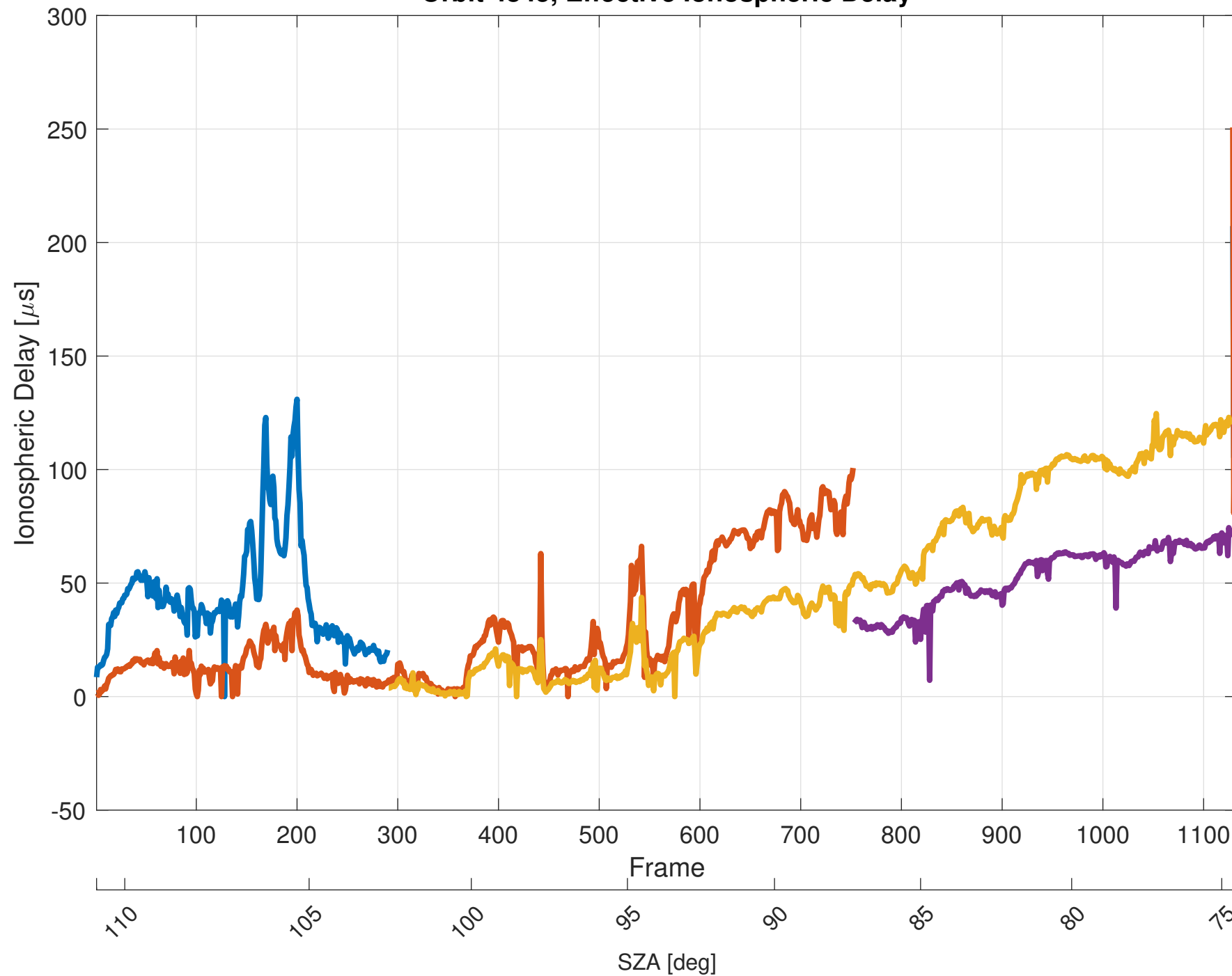
Orbit 4845, Effective Ionospheric Delay
