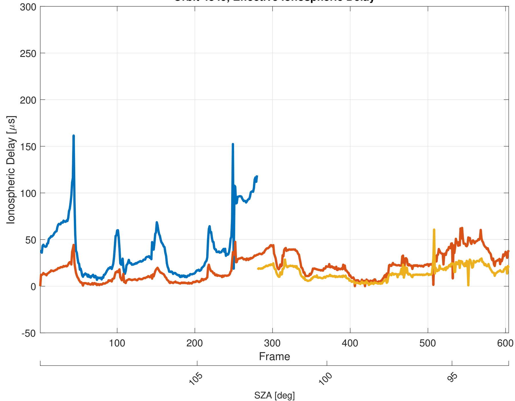
Orbit 4849, Effective Ionospheric Delay
