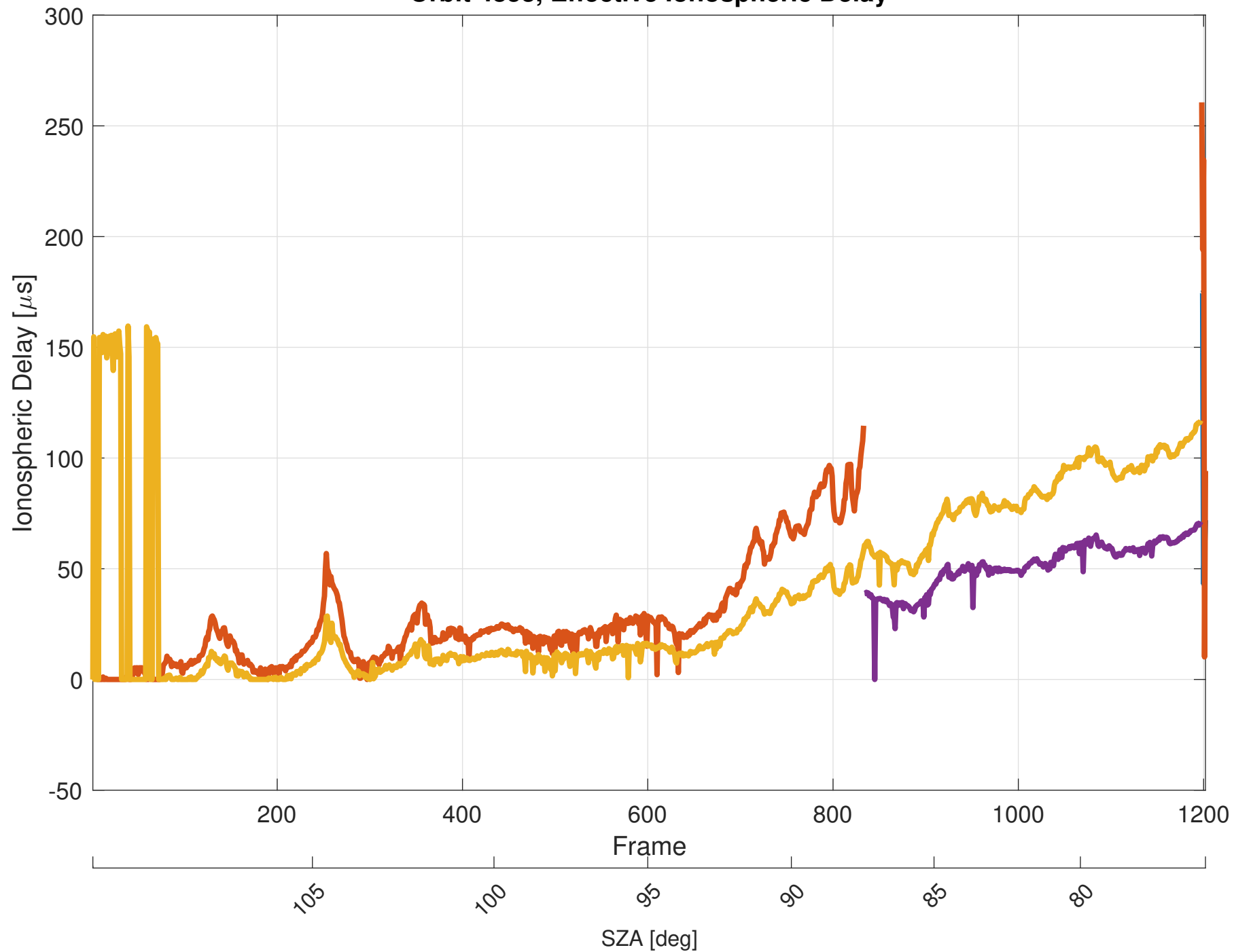
Orbit 4853, Effective Ionospheric Delay
