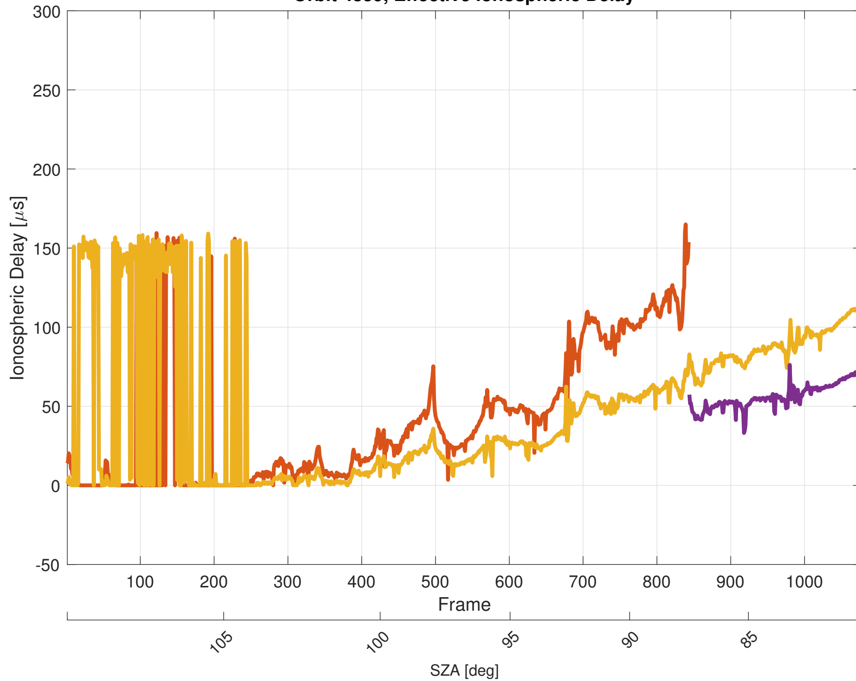
Orbit 4859, Effective Ionospheric Delay
