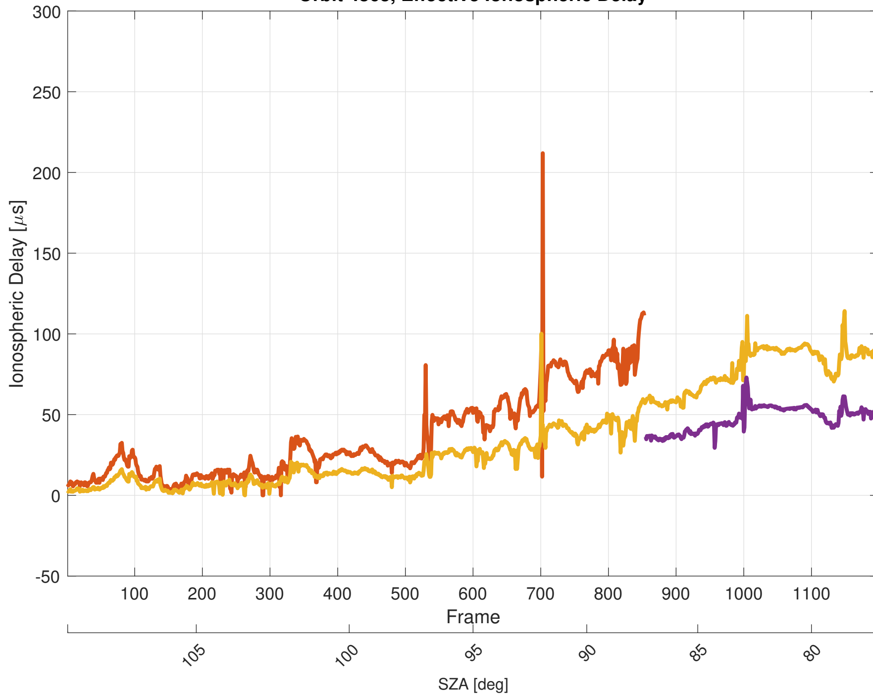
Orbit 4863, Effective Ionospheric Delay
